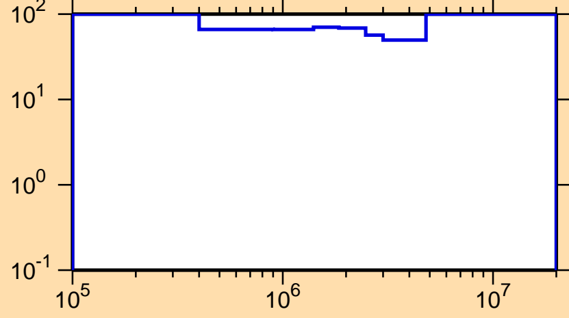
\Delta\sigma/\sigma vs. E for ^{218}\text{At}(n,\text{inel.})
