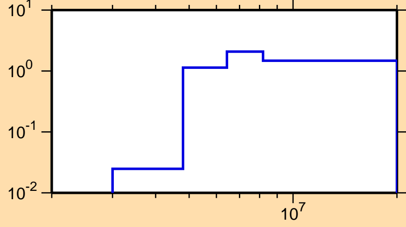
\sigma vs. E for ^{218}\text{At}(n,2n)
