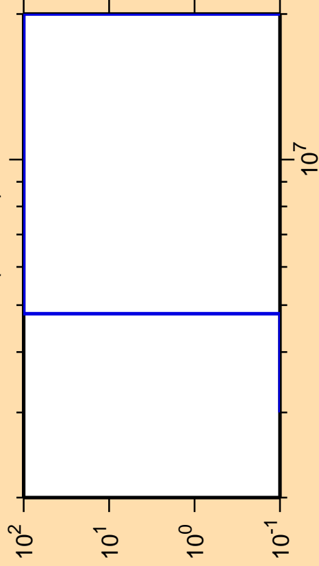
\Delta\sigma/\sigma vs. E for ^{218}\text{At}(n,2n\alpha)
