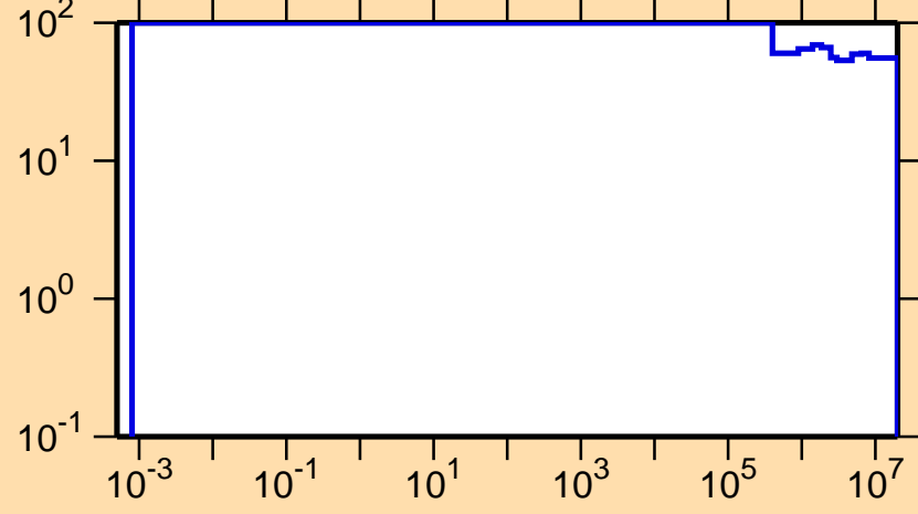
\Delta\sigma/\sigma vs. E for ^{218}\text{At}(n,\text{nonel.})
