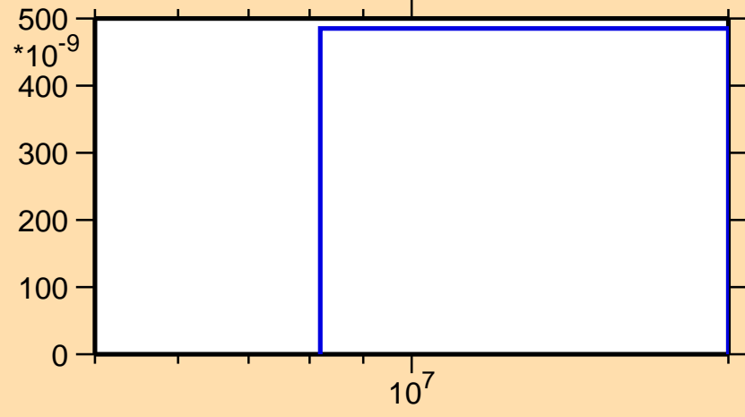
\sigma vs. E for ^{218}\text{At}(n,2np)
