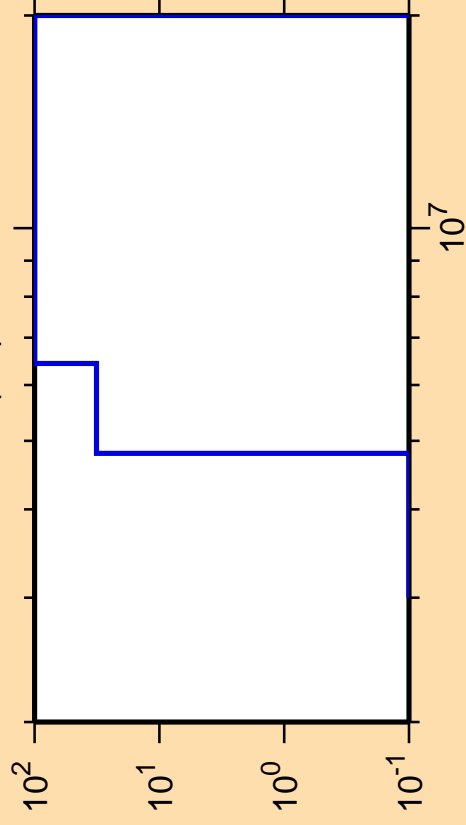
\Delta\sigma/\sigma vs. E for ^{218}\text{At}(n,t)
