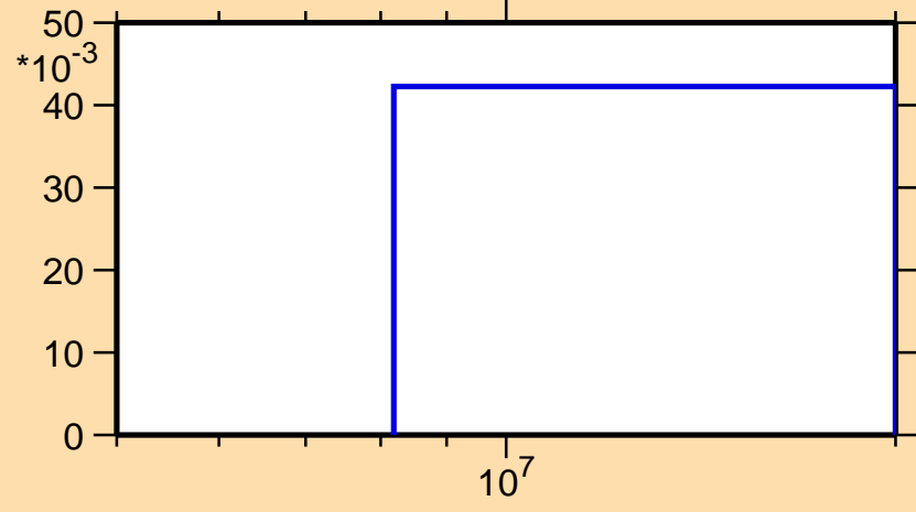
\sigma vs. E for ^{218}\text{At}(n,3n\alpha)
