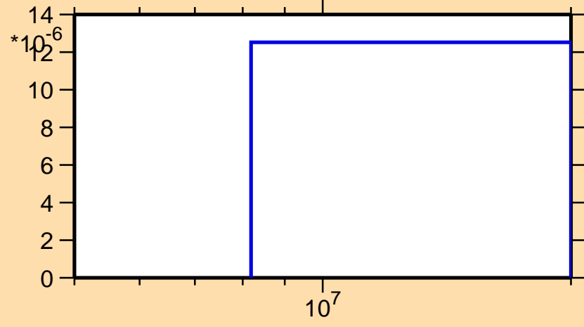
\sigma vs. E for ^{218}\text{At}(n,nt)
