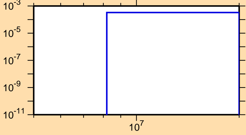
\sigma vs. E for ^{218}\text{At}(n,np)
