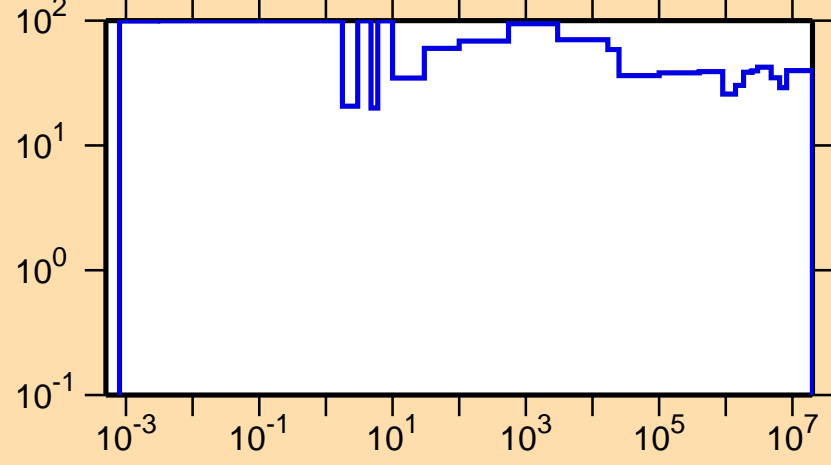
\Delta\sigma/\sigma vs. E for ^{218}\text{At}(n,\text{tot.})
