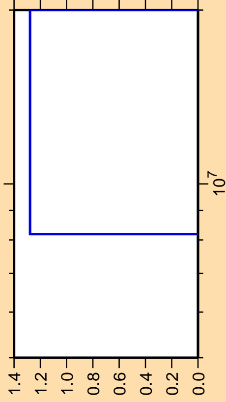
\Delta\sigma/\sigma vs. E for ^{218}\text{At}(\text{mt } 42)
