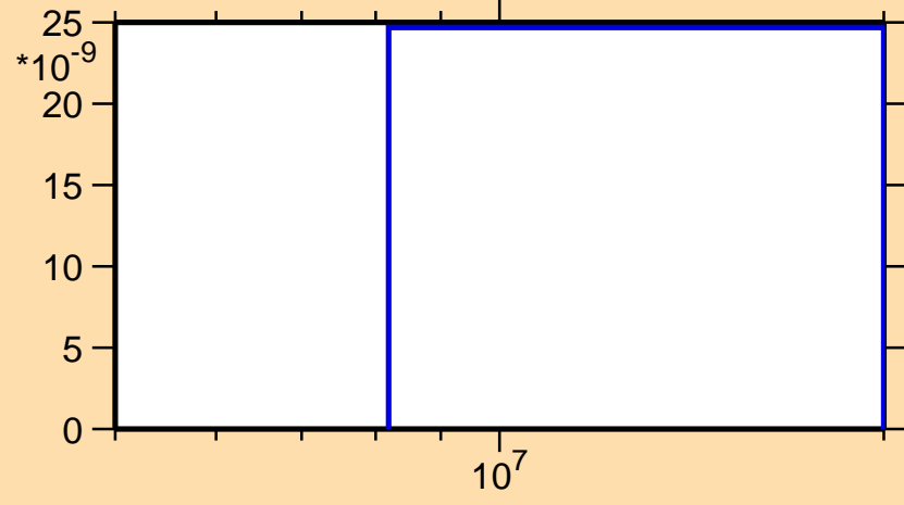
\sigma vs. E for ^{218}\text{At}(\text{mt117})
