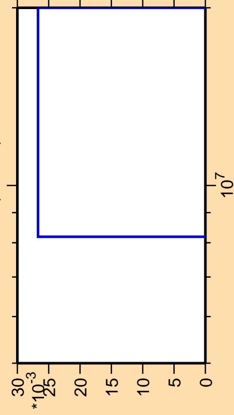
\Delta\sigma/\sigma vs. E for ^{218}\text{At}(\text{mt } 34)
