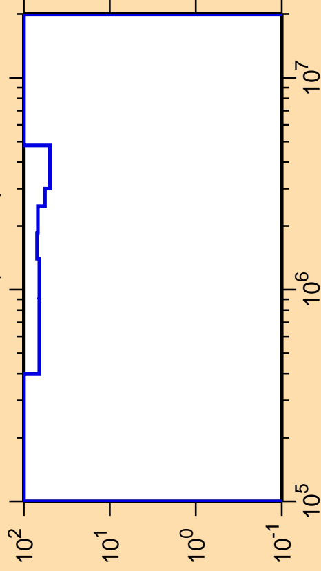
\Delta\sigma/\sigma vs. E for ^{218}\text{At}(n,\text{inel.})
