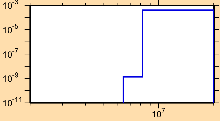
\sigma vs. E for ^{218}\text{At}(n,t)
