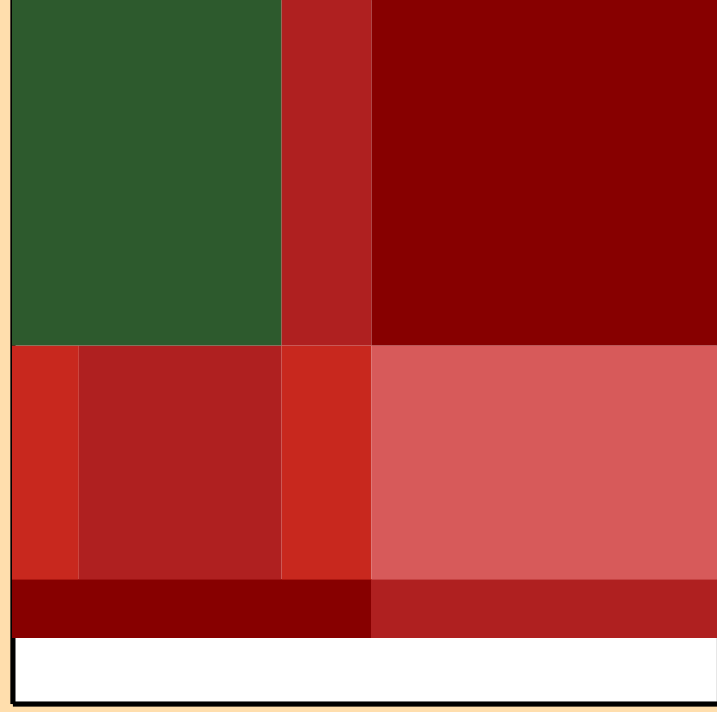
\Delta\sigma/\sigma vs. E for ^{218}\text{At}(n,\text{inel.})
