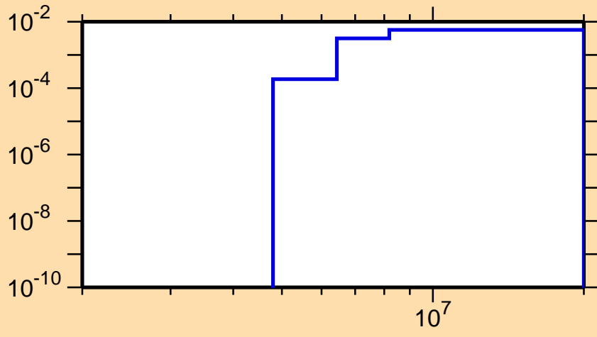
\sigma vs. E for ^{218}\text{At}(n,2n\alpha)
