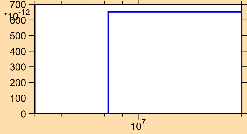
\sigma vs. E for ^{218}\text{At}(n,p\alpha)
