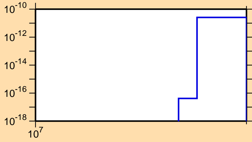
\sigma vs. E for ^{219}\text{At}(\text{mt } 42)
