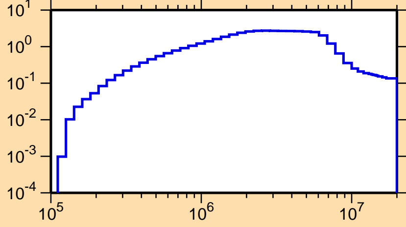
\sigma vs. E for ^{219}\text{At}(n,\text{inel.})
