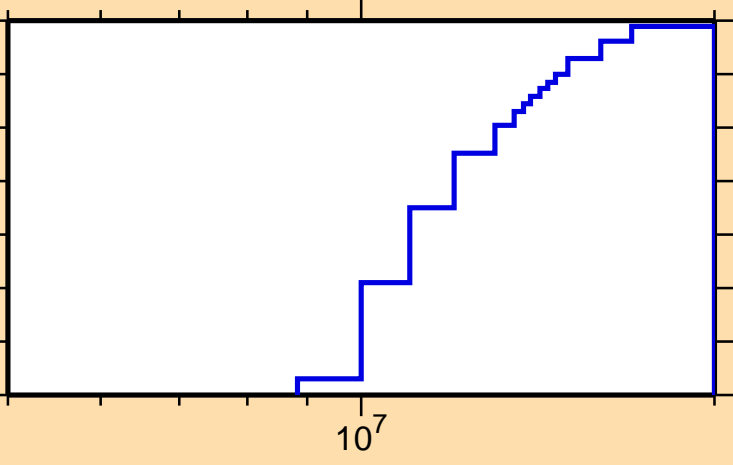
\sigma vs. E for ^{219}\text{At}(\text{mt117})
