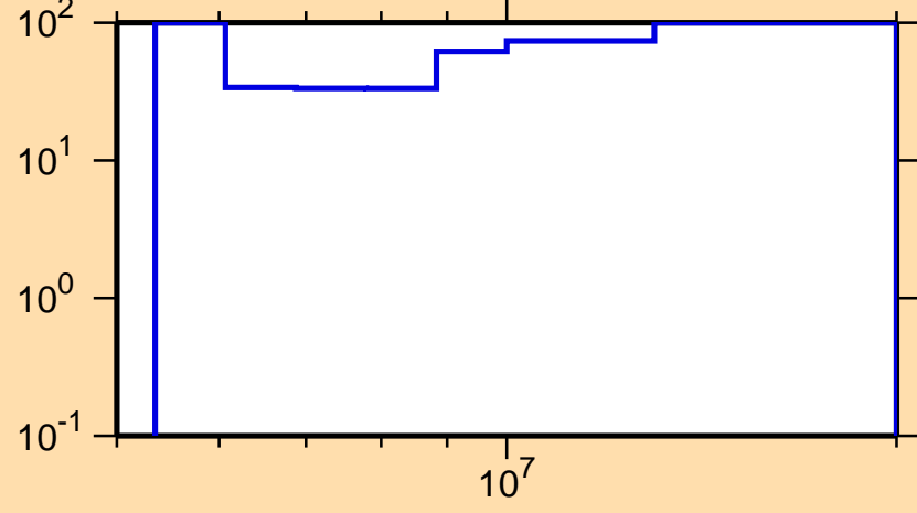
\Delta\sigma/\sigma vs. E for ^{219}\text{At}(n,2n)
