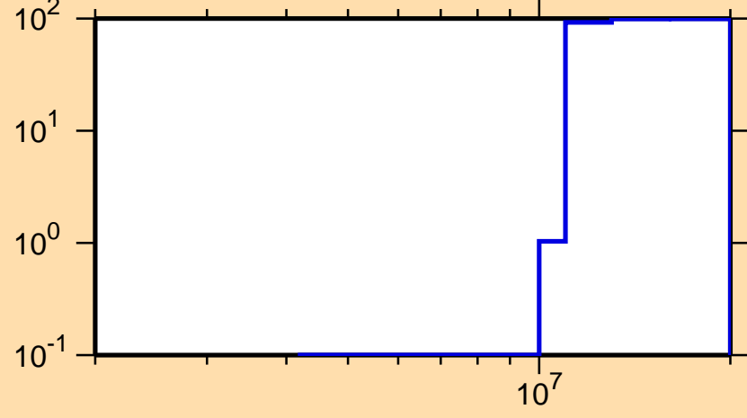
\Delta\sigma/\sigma vs. E for ^{219}\text{At}(n,f)
