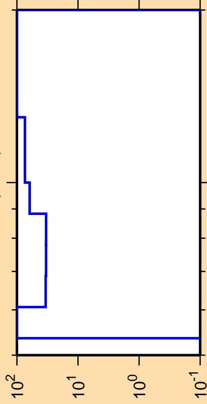
\Delta\sigma/\sigma vs. E for ^{219}\text{At}(n,2n)
