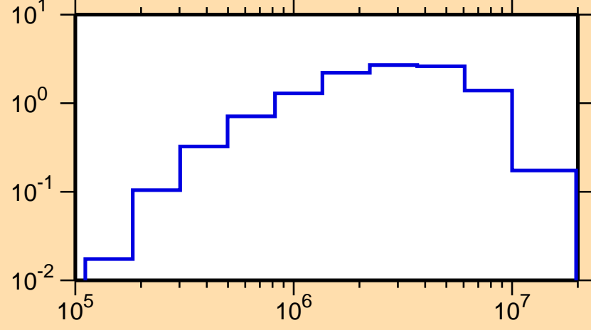
\sigma vs. E for ^{219}\text{At}(n,n\text{cont.})
