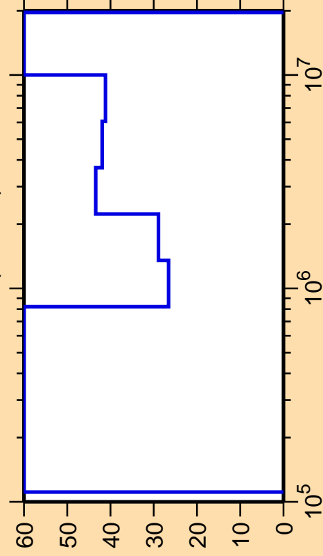
\Delta\sigma/\sigma vs. E for ^{219}\text{At}(n,\text{inel.})
