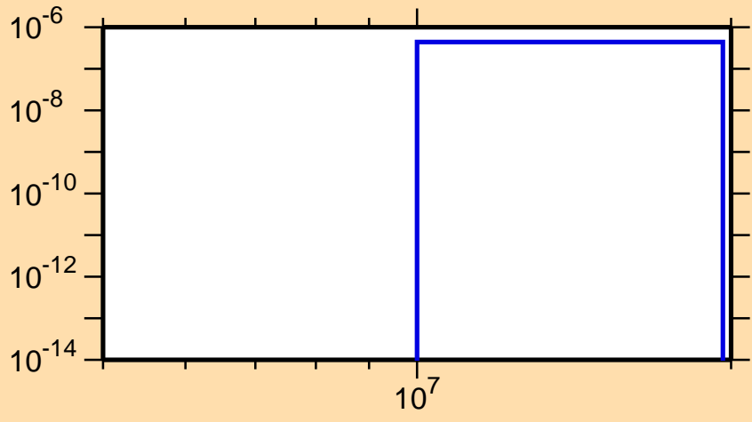
\sigma vs. E for ^{219}\text{At}(n,\text{nd})
