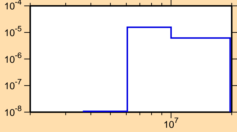
\sigma vs. E for ^{219}\text{At}(n,2n\alpha)
