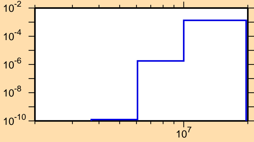
\sigma vs. E for ^{219}\text{At}(n,p)
