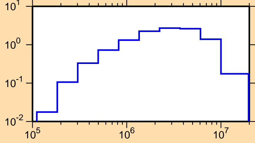
\sigma vs. E for ^{219}\text{At}(n,\text{inel.})
