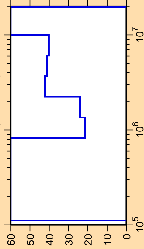
\Delta\sigma/\sigma vs. E for ^{219}\text{At}(n,\text{ncont.})
