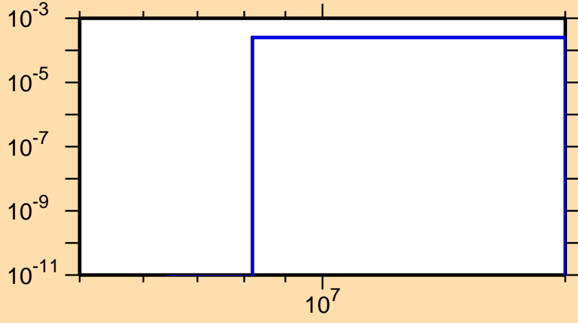
\sigma vs. E for ^{219}\text{At}(n,d)
