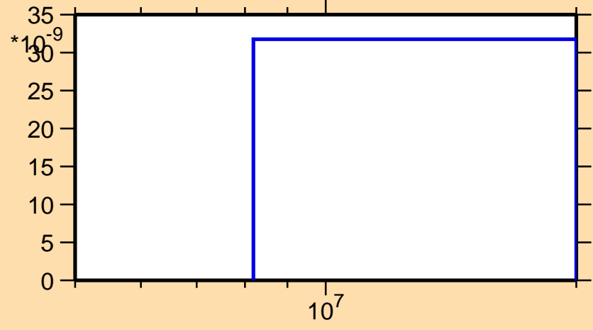
\sigma vs. E for ^{219}\text{At}(\text{mt } 45)
