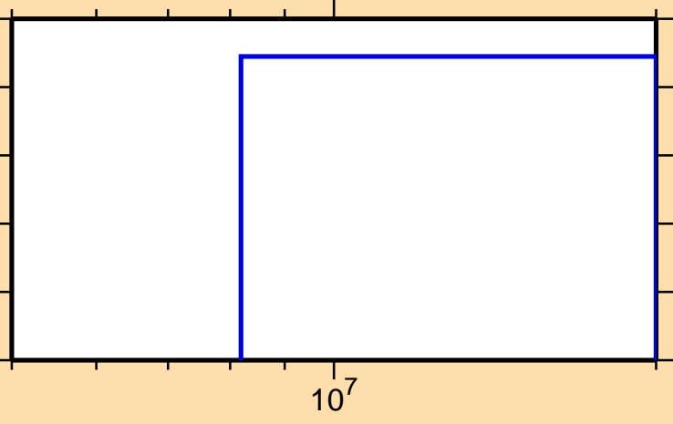
\sigma vs. E for ^{219}\text{At}(n,\text{He}3)
