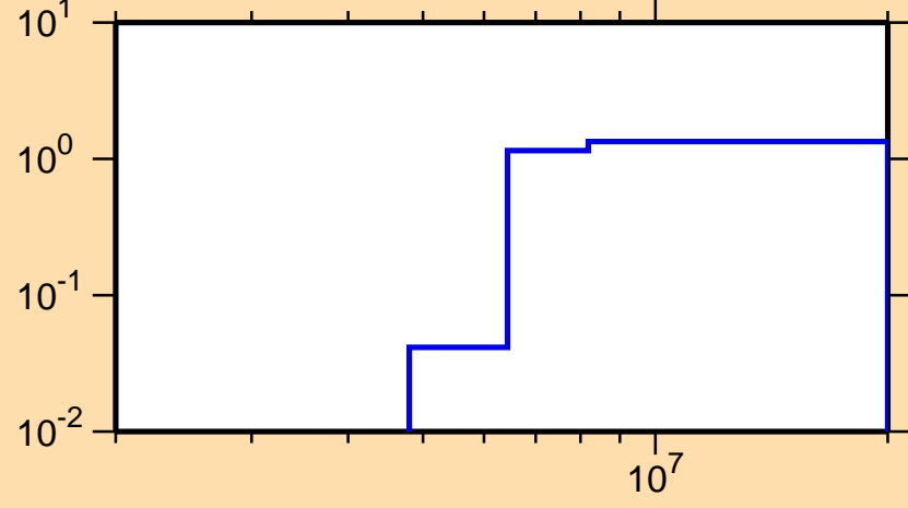
\sigma vs. E for ^{219}\text{At}(n,2n)
