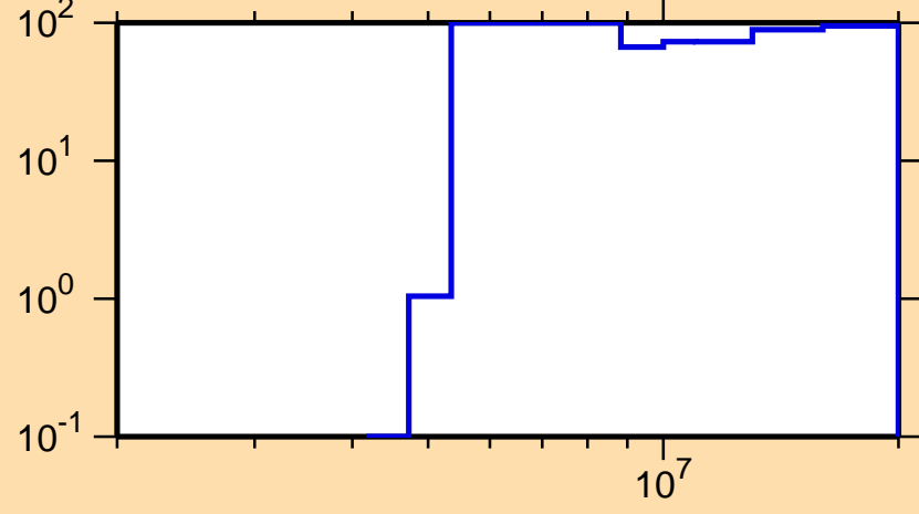
\Delta\sigma/\sigma vs. E for ^{221}\text{At}(n,p)
