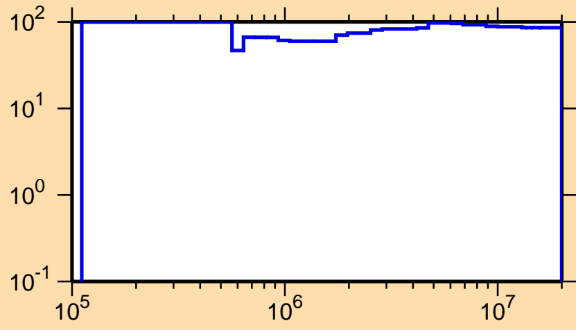
\Delta\sigma/\sigma vs. E for ^{221}\text{At}(n,n\text{cont.})
