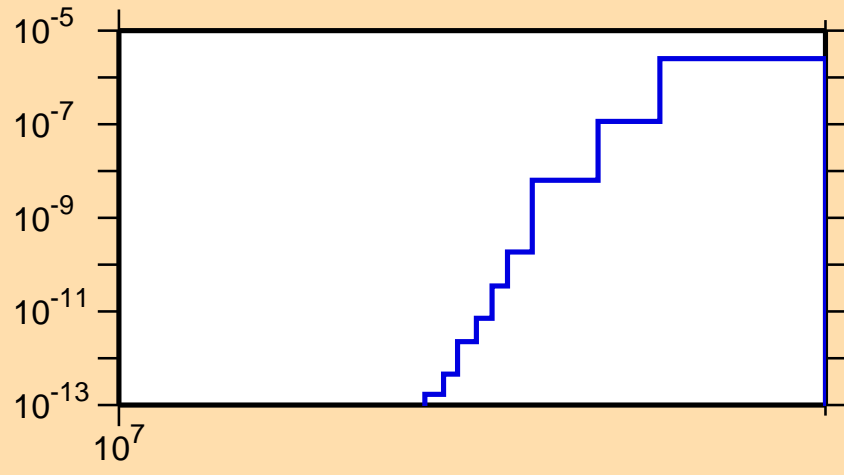
\sigma vs. E for ^{221}\text{At}(n,2np)
