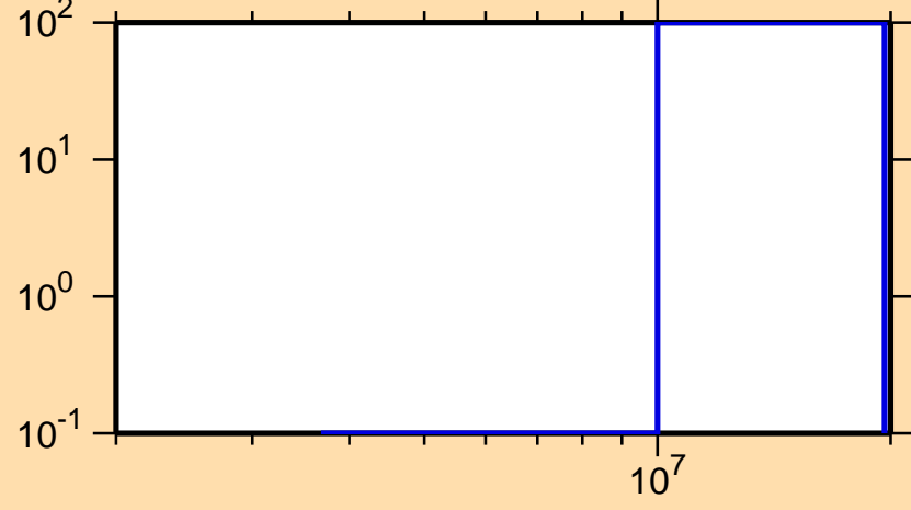
\Delta\sigma/\sigma vs. E for ^{221}\text{At}(n,f)
