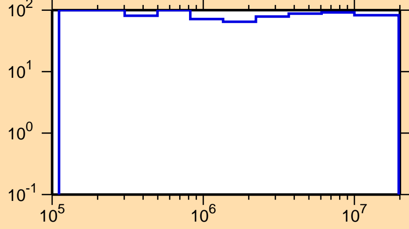
\Delta\sigma/\sigma vs. E for ^{221}\text{At}(n,\text{inel.})
