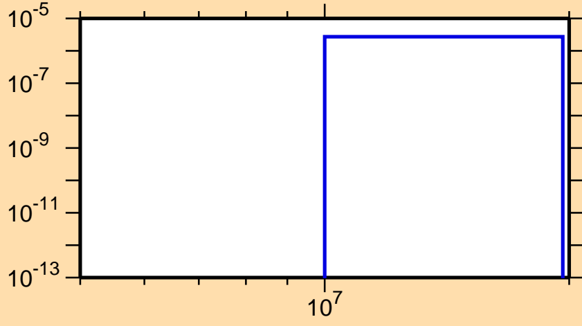
\sigma vs. E for ^{221}\text{At}(n,nt)
