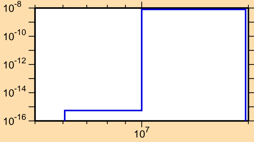
\sigma vs. E for ^{221}\text{At}(n,3n\alpha)
