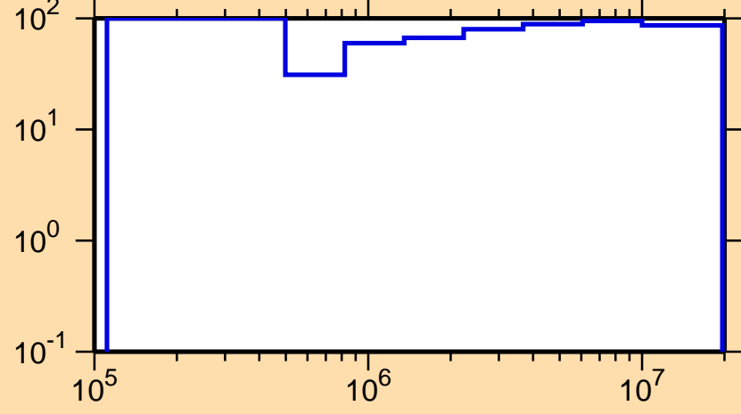
\Delta\sigma/\sigma vs. E for ^{221}\text{At}(n,ncont.)
