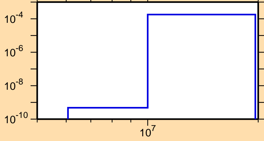
\sigma vs. E for ^{221}\text{At}(n,d)
