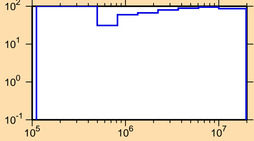
\Delta\sigma/\sigma vs. E for ^{221}\text{At}(n,n\text{cont.})
