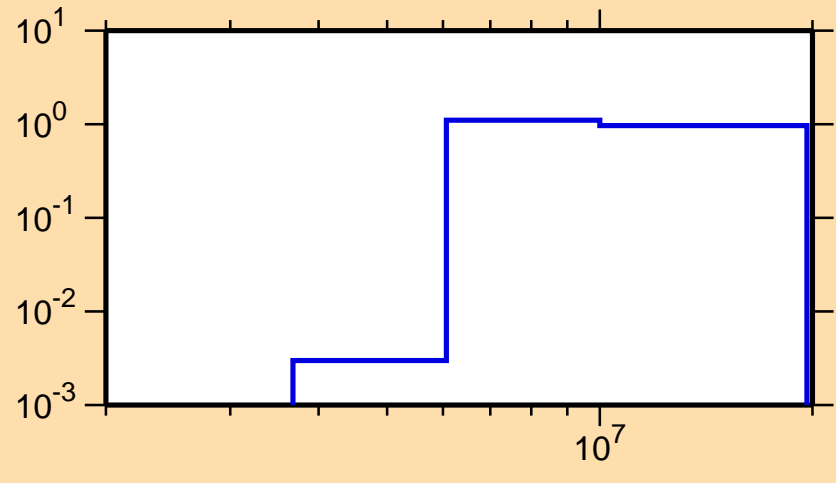
\sigma vs. E for ^{221}\text{At}(n,2n)
