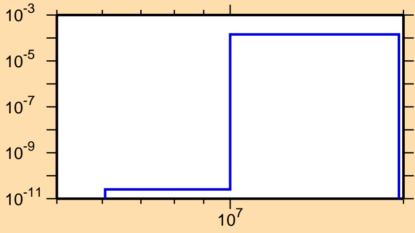
\sigma vs. E for ^{221}\text{At}(n,np)
