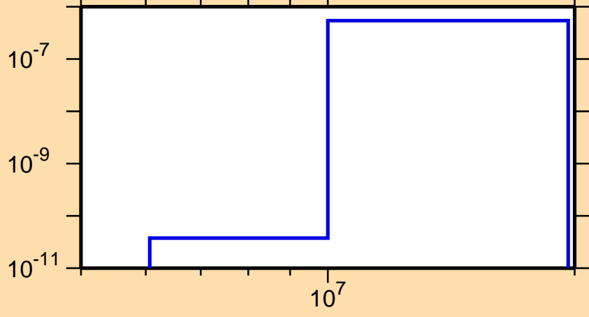
\sigma vs. E for ^{221}\text{At}(n,2n\alpha)
