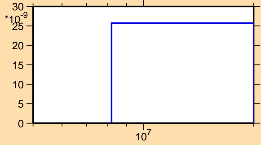
\sigma vs. E for ^{221}\text{At}(n,2np)
