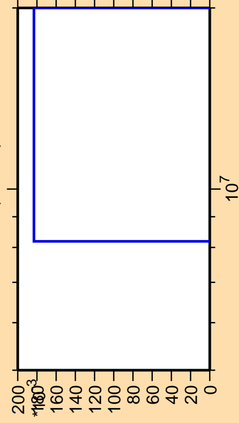
\Delta\sigma/\sigma vs. E for ^{221}\text{At}(\text{mt } 42)
