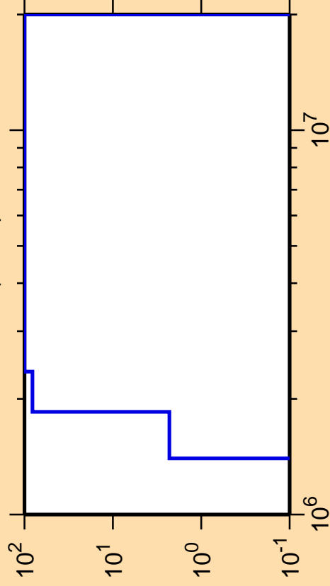
\Delta\sigma/\sigma vs. E for ^{221}\text{At}(n,n\alpha)
