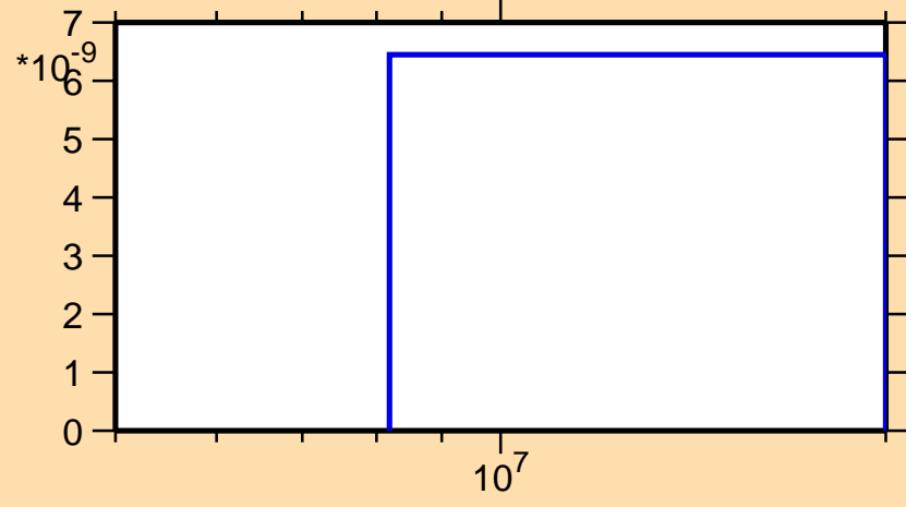
\sigma vs. E for ^{221}\text{At}(n,3n\alpha)
