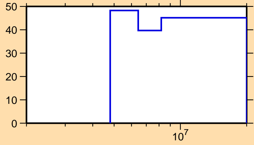
\Delta\sigma/\sigma vs. E for ^{221}\text{At}(n,\text{tot.})
