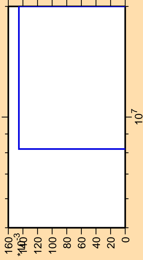
\Delta\sigma/\sigma vs. E for ^{221}\text{At}(n,\text{He}3)
