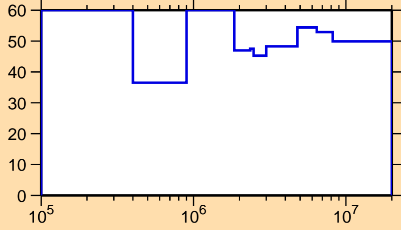
\Delta\sigma/\sigma vs. E for ^{221}\text{At}(n,\text{el.})
