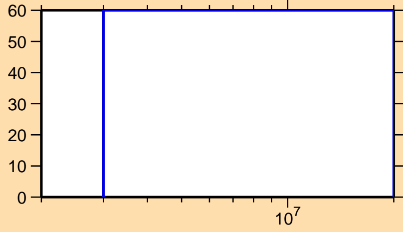
\Delta\sigma/\sigma vs. E for ^{221}\text{At}(n,\gamma)
