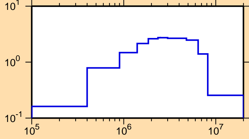
\sigma vs. E for ^{221}\text{At}(n,\text{inel.})
