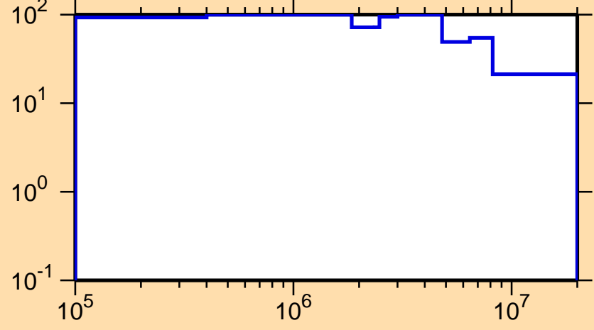
\Delta\sigma/\sigma vs. E for ^{221}\text{At}(n,n_1)
