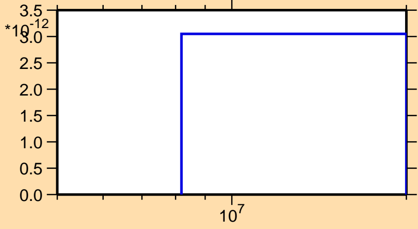
\sigma vs. E for ^{221}\text{At}(\text{mt } 11)
