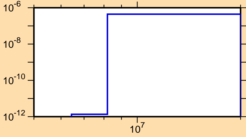
\sigma vs. E for ^{221}\text{At}(n,2n\alpha)
