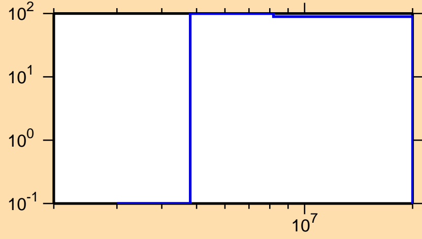
\Delta\sigma/\sigma vs. E for ^{221}\text{At}(n,p)
