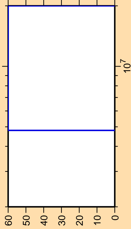
\Delta\sigma/\sigma vs. E for ^{221}\text{At}(n,n\text{cont.})
