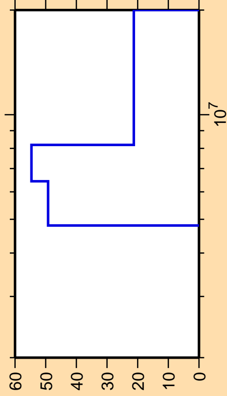
\Delta\sigma/\sigma vs. E for ^{221}\text{At}(n,n_1)
