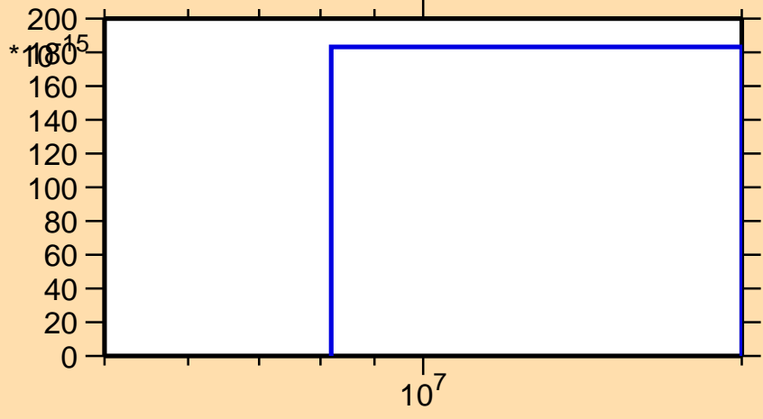
\sigma vs. E for ^{221}\text{At}(\text{mt } 42)
