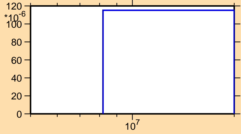
\sigma vs. E for ^{221}\text{At}(n,np)
