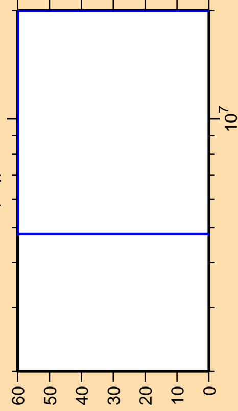
\Delta\sigma/\sigma vs. E for ^{221}\text{At}(n,\gamma)
