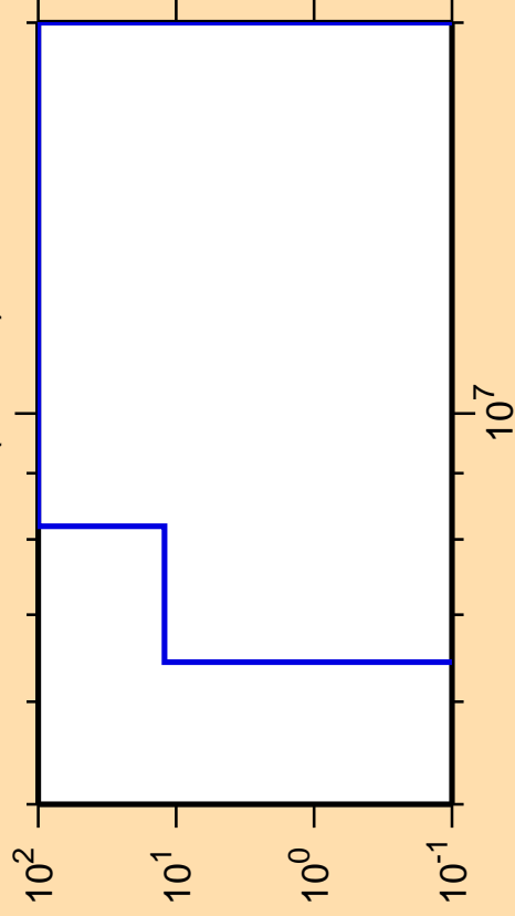
\Delta\sigma/\sigma vs. E for ^{221}\text{At}(n,2n\alpha)
