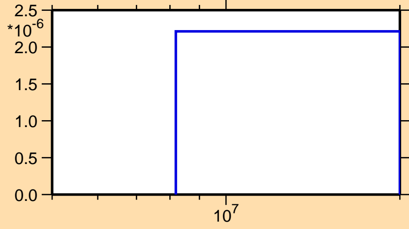
\sigma vs. E for ^{221}\text{At}(n,nt)
