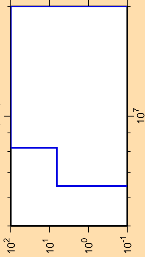
\Delta\sigma/\sigma vs. E for ^{221}\text{At}(n,d)
