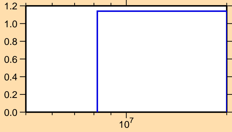
\sigma vs. E for ^{221}\text{At}(n,3n)
