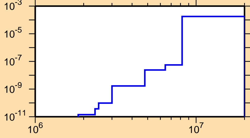
\sigma vs. E for ^{221}\text{At}(n,n\alpha)
