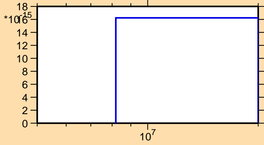
\sigma vs. E for ^{221}\text{At}(n,\text{He}3)
