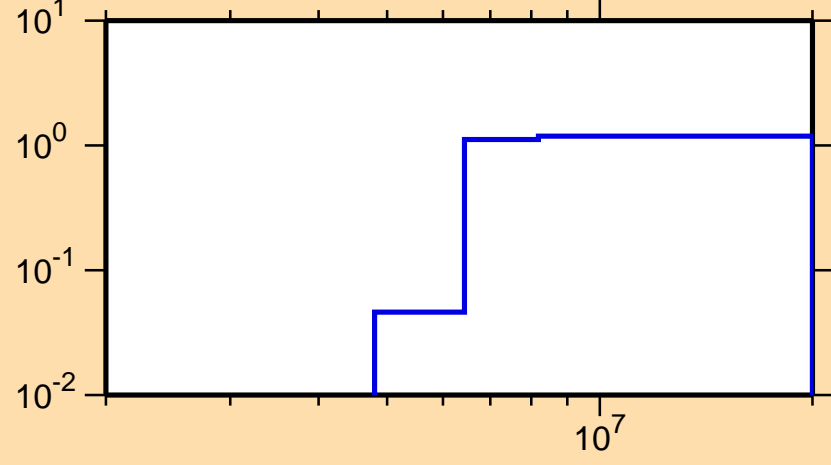
\sigma vs. E for ^{221}\text{At}(n,2n)
