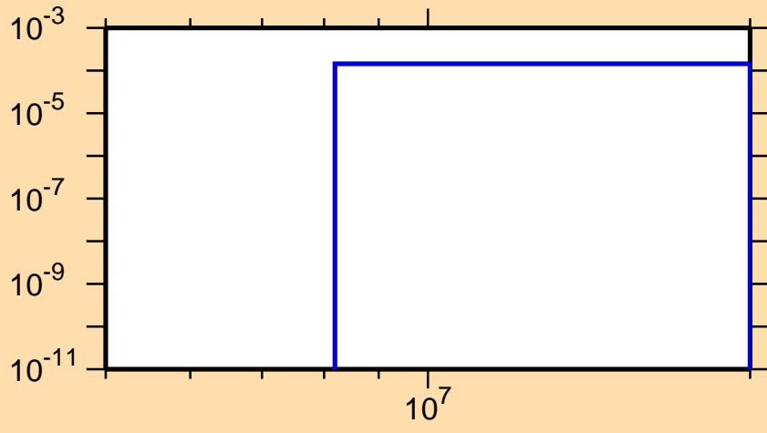
\sigma vs. E for ^{221}\text{At}(n,d)
