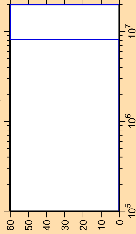
\Delta\sigma/\sigma vs. E for ^{221}\text{At}(n,f)
