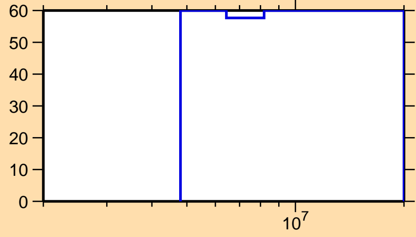
\Delta\sigma/\sigma vs. E for ^{221}\text{At}(n,\text{nonel.})
