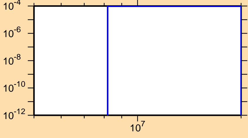
\sigma vs. E for ^{221}\text{At}(n,t)
