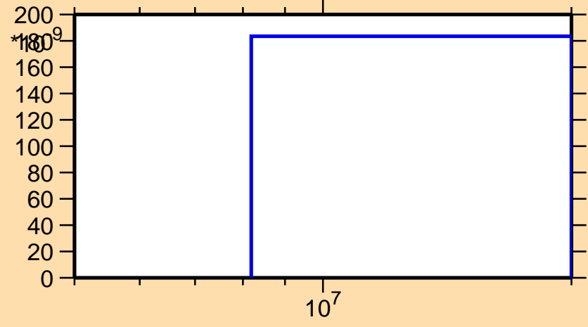
\sigma vs. E for ^{221}\text{At}(n,\text{nd})
