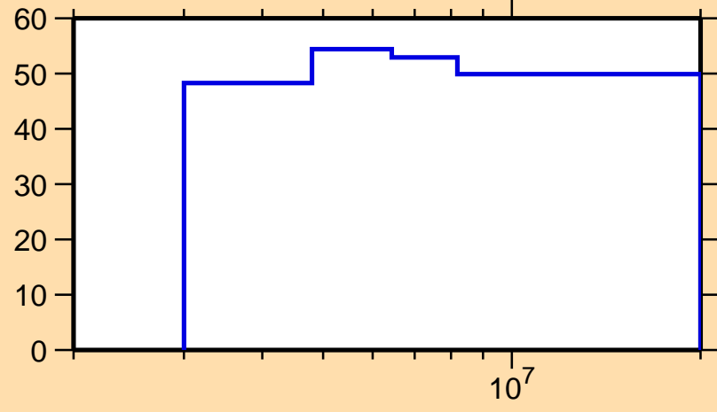
\Delta\sigma/\sigma vs. E for ^{221}\text{At}(n,el.)
