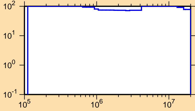
\Delta\sigma/\sigma vs. E for ^{222}\text{At}(n,ncont.)
