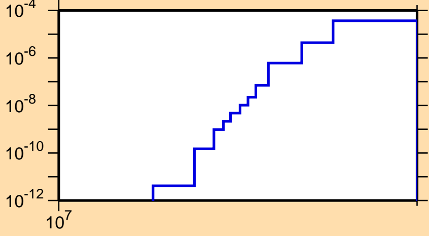
\sigma vs. E for ^{222}\text{At}(n,2np)
