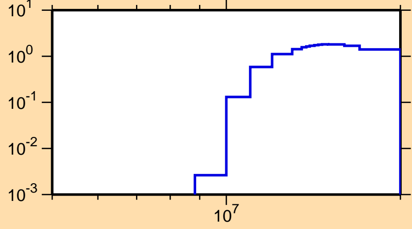
\sigma vs. E for ^{222}\text{At}(n,3n)
