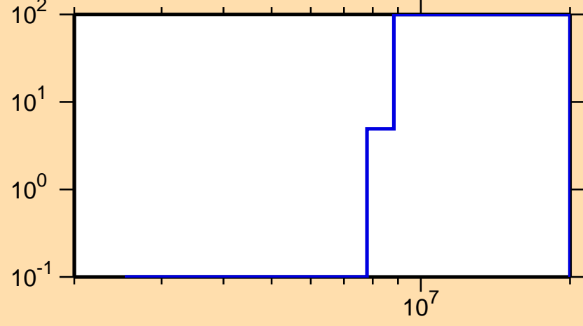
\Delta\sigma/\sigma vs. E for ^{222}\text{At}(n,f)
