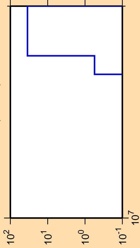
\Delta\sigma/\sigma vs. E for ^{222}\text{At}(n,\text{He}3)
