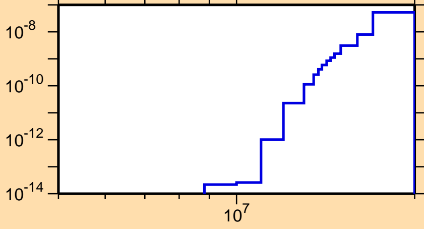
\sigma vs. E for ^{222}\text{At}(n,3n\alpha)
