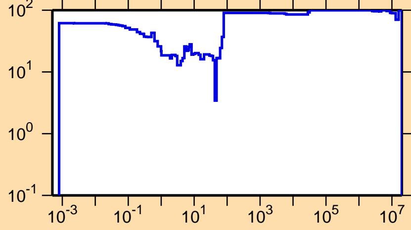
\Delta\sigma/\sigma vs. E for ^{222}\text{At}(n,\gamma)
