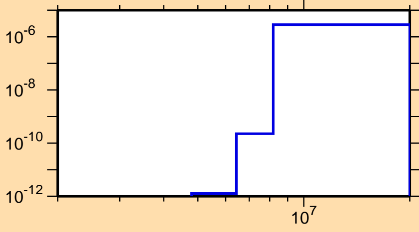
\sigma vs. E for ^{222}\text{At}(n,2n\alpha)
