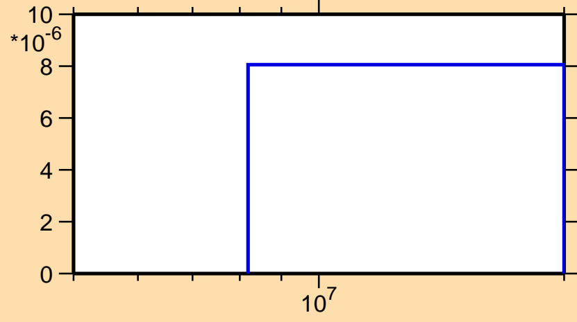
\sigma vs. E for ^{222}\text{At}(n,nt)
