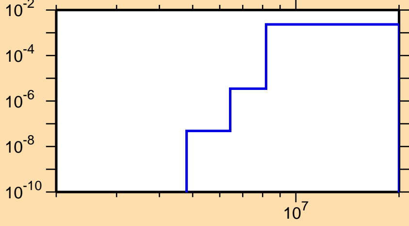
\sigma vs. E for ^{222}\text{At}(n,p)
