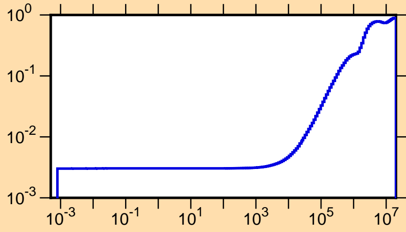
\mu vs. E for ^{223}\text{At}(\text{mt251})
