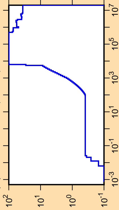
\Delta\mu/\mu vs. E for ^{223}\text{At}(\text{mt251})
