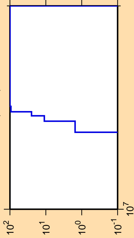
\Delta\sigma/\sigma vs. E for ^{223}\text{At}(n,nd)
