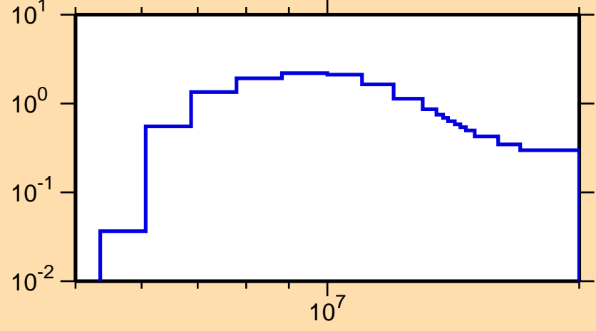
\sigma vs. E for ^{223}\text{At}(n,2n)
