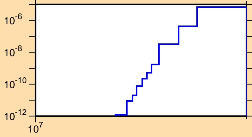
\sigma vs. E for ^{223}\text{At}(n,nd)
