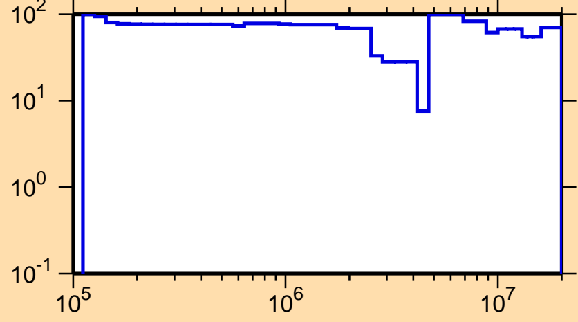
\Delta\sigma/\sigma vs. E for ^{223}\text{At}(n,n_1)
