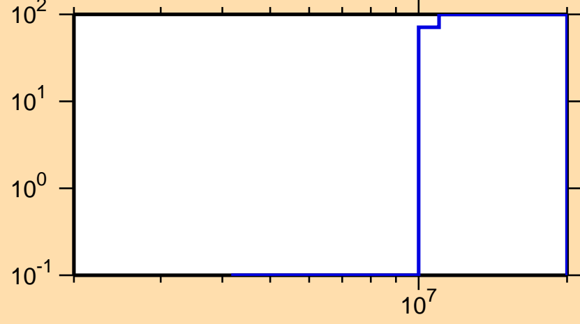
\Delta\sigma/\sigma vs. E for ^{223}\text{At}(n,f)
