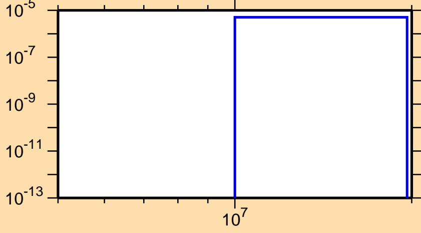
\sigma vs. E for ^{223}\text{At}(n,nt)
