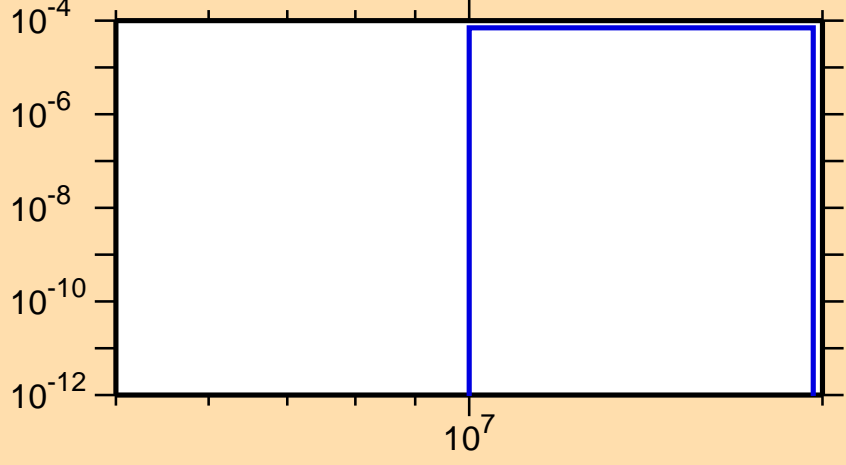
\sigma vs. E for ^{223}\text{At}(n,np)
