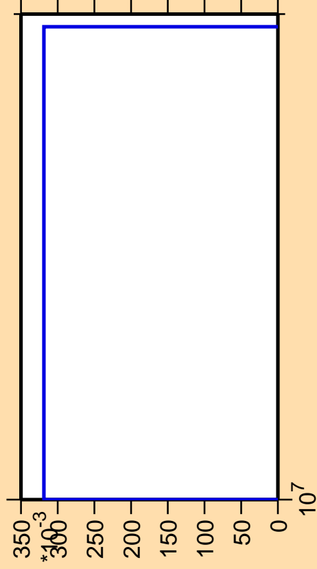
\Delta\sigma/\sigma vs. E for ^{223}\text{At}(\text{mt } 42)
