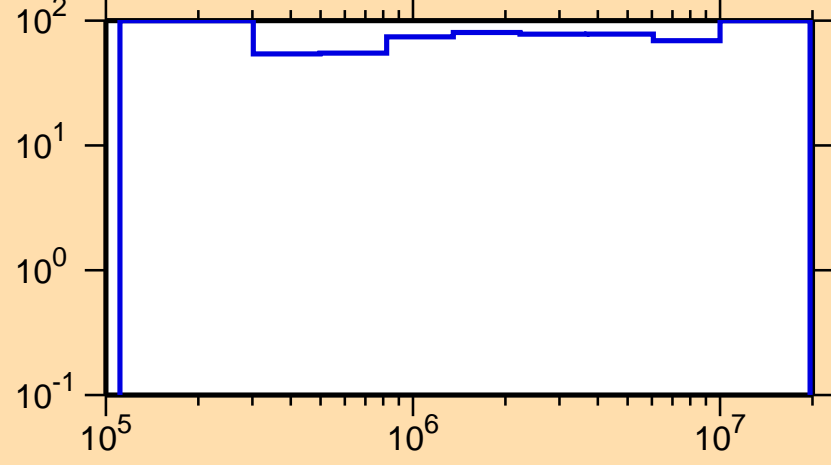
\Delta\sigma/\sigma vs. E for ^{223}\text{At}(n,ncont.)
