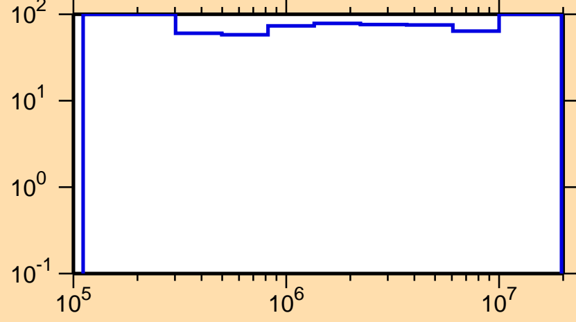
\Delta\sigma/\sigma vs. E for ^{223}\text{At}(n,\text{inel.})
