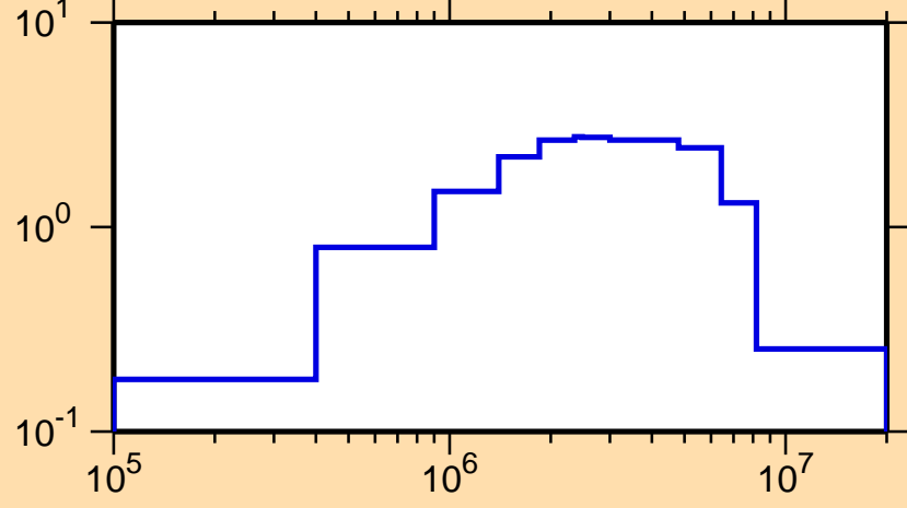
\sigma vs. E for ^{223}\text{At}(n,\text{inel.})
