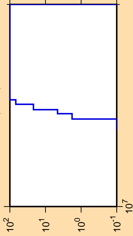
\Delta\sigma/\sigma vs. E for ^{225}\text{At}(n,nd)
