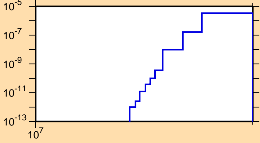
\sigma vs. E for ^{225}\text{At}(n,nd)
