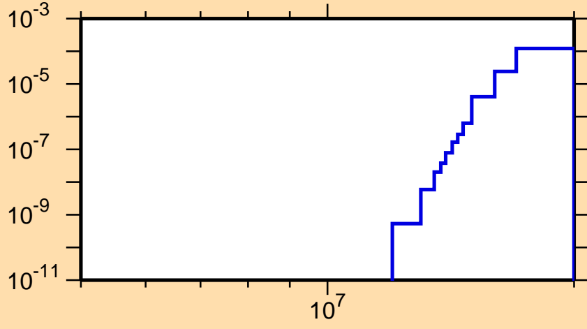
\sigma vs. E for ^{225}\text{At}(n,nt)
