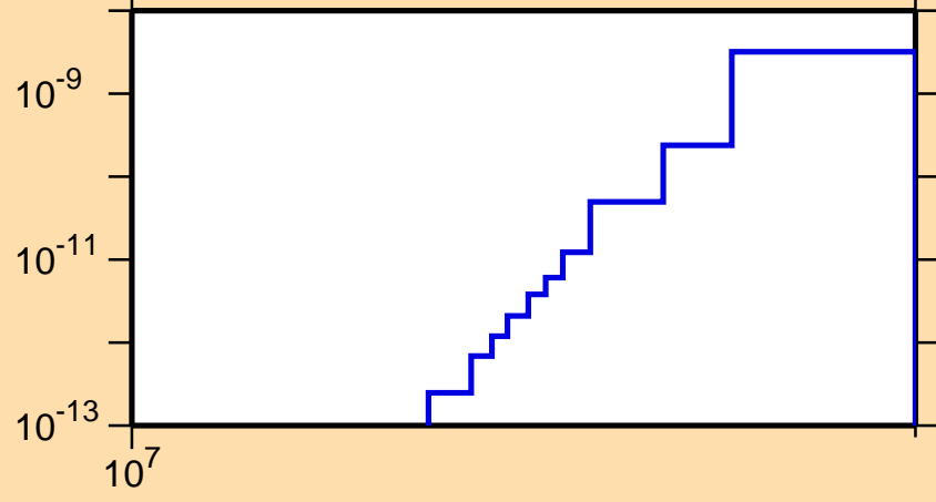
\sigma vs. E for ^{225}\text{At}(n,3n\alpha)
