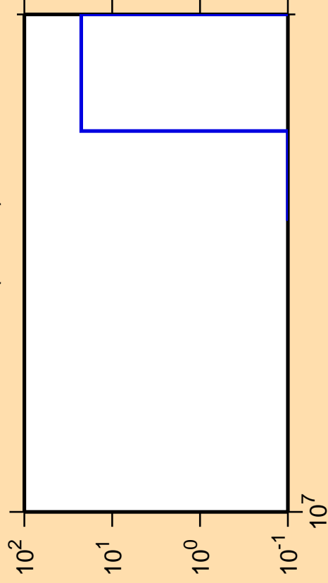
\Delta\sigma/\sigma vs. E for ^{225}\text{At} (mt 42)
