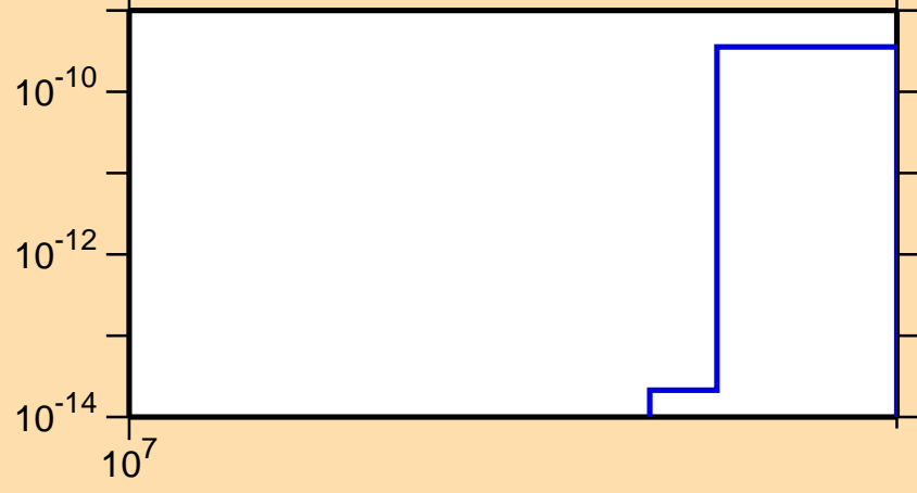
\sigma vs. E for ^{225}\text{At}(\text{mt } 11)
