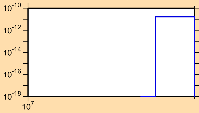
\sigma vs. E for ^{225}\text{At} (mt 42)
