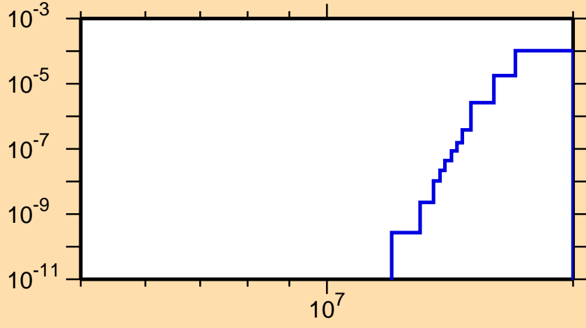
\sigma vs. E for ^{226}\text{At}(n,nt)
