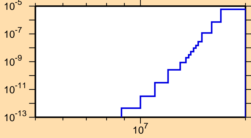
\sigma vs. E for ^{226}\text{At}(n,2n\alpha)
