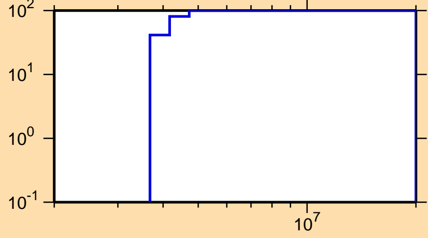
\Delta\sigma/\sigma vs. E for ^{226}\text{At}(n,\text{inel.})
