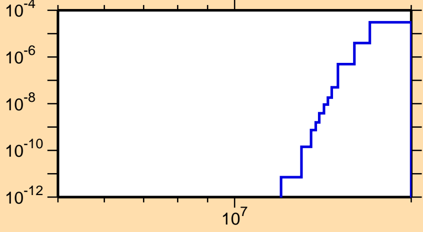
\sigma vs. E for ^{226}\text{At}(n,\text{nd})
