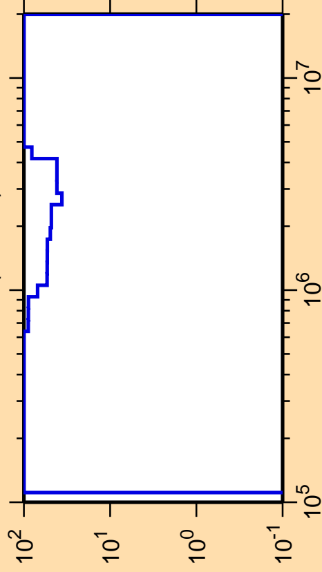
\Delta\sigma/\sigma vs. E for ^{226}\text{At}(n,\text{inel.})
