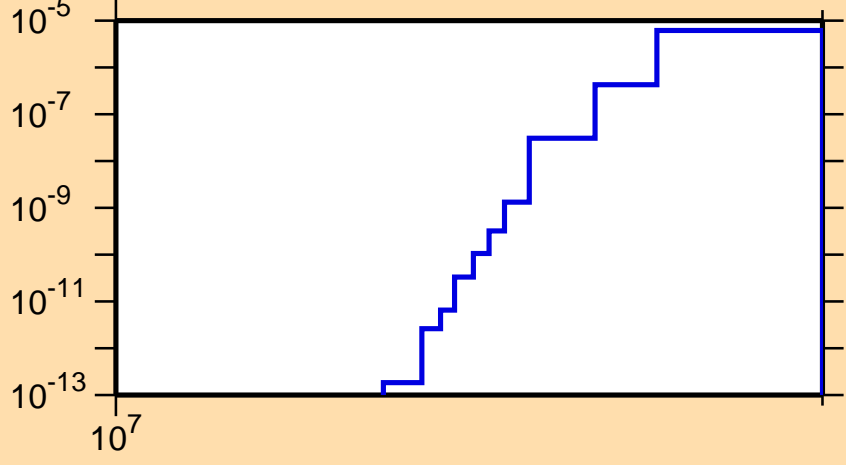
\sigma vs. E for ^{226}\text{At}(n,2np)
