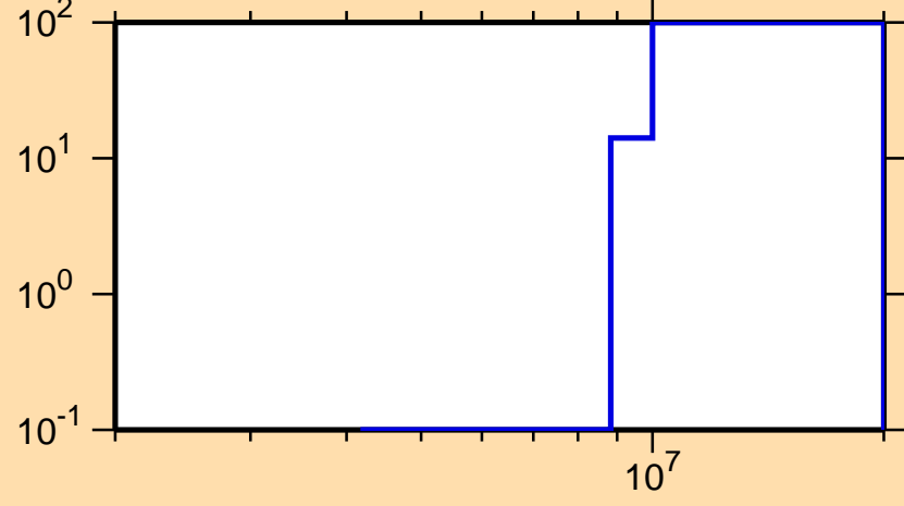
\Delta\sigma/\sigma vs. E for ^{226}\text{At}(n,f)
