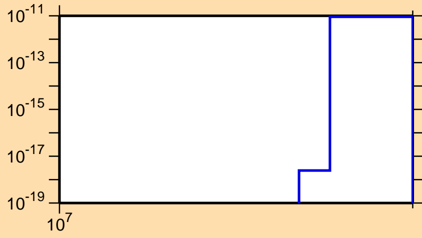
\sigma vs. E for ^{226}\text{At}(\text{mt } 42)
