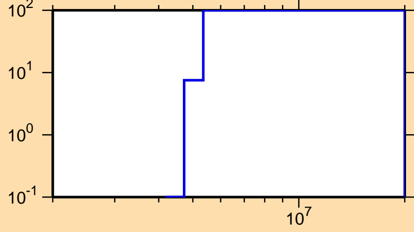
\Delta\sigma/\sigma vs. E for ^{226}\text{At}(n,p)
