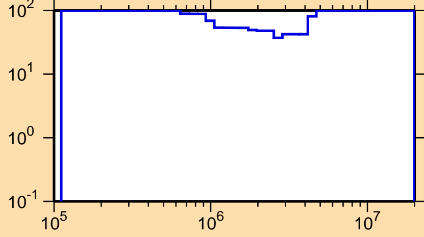
\Delta\sigma/\sigma vs. E for ^{226}\text{At}(n,n\text{cont.})
