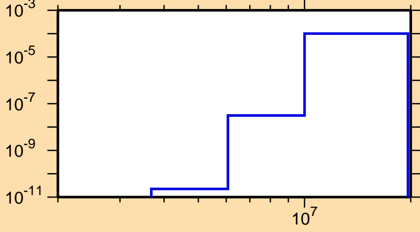
\sigma vs. E for ^{226}\text{At}(n,\alpha)
