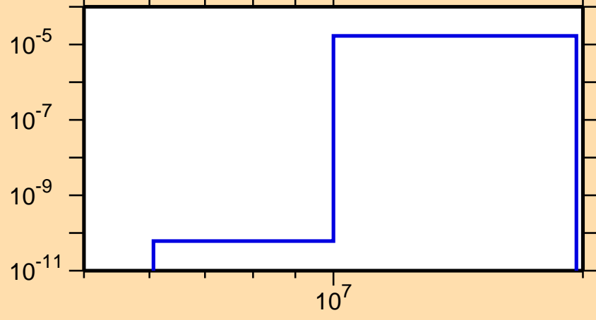
\sigma vs. E for ^{226}\text{At}(n,n\alpha)
