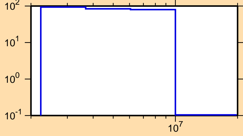
\Delta\sigma/\sigma vs. E for ^{226}\text{At}(n,n_1)
