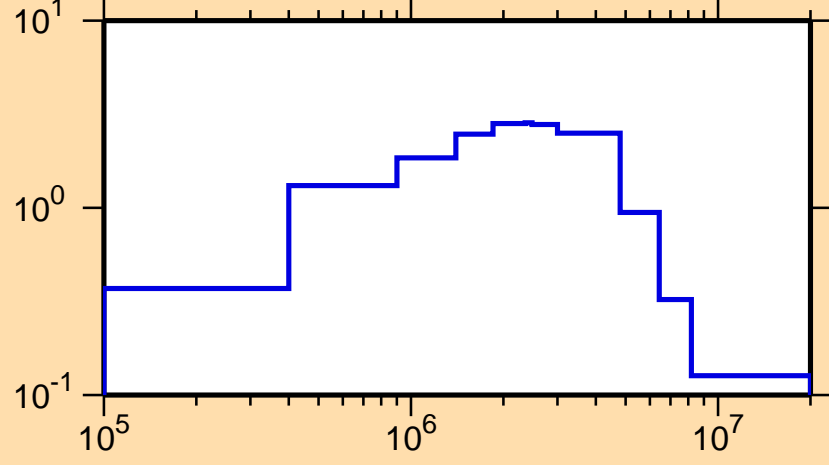
\sigma vs. E for ^{226}\text{At}(n,\text{inel.})
