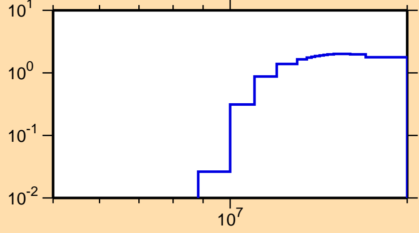
\sigma vs. E for ^{227}\text{At}(n,3n)
