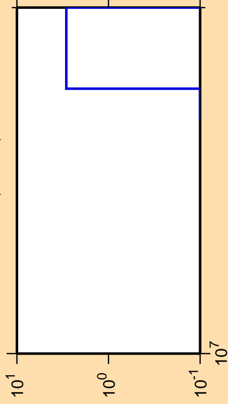
\Delta\sigma/\sigma vs. E for ^{227}\text{At}(\text{mt } 42)
