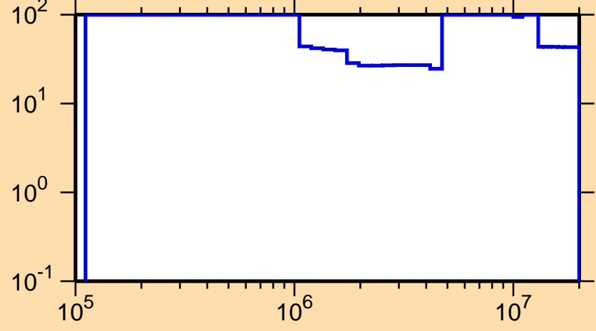
\Delta\sigma/\sigma vs. E for ^{227}\text{At}(n,\text{inel.})
