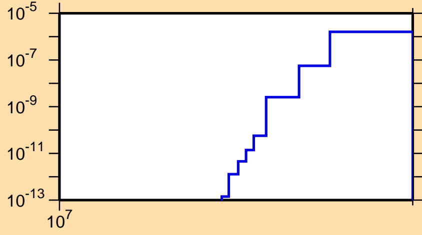
\sigma vs. E for ^{227}\text{At}(n,\text{nd})
