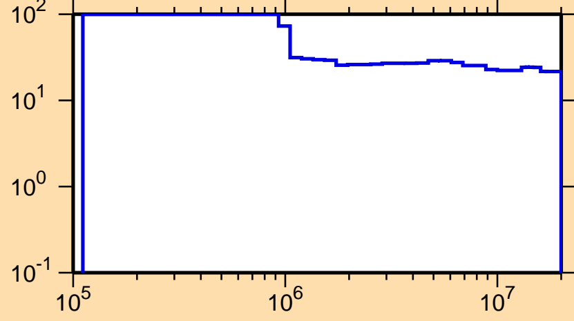
\Delta\sigma/\sigma vs. E for ^{227}\text{At}(n,\text{nonel.})
