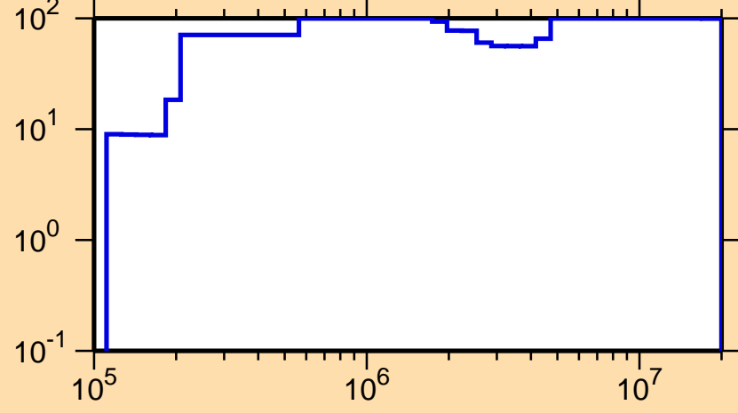
\Delta\sigma/\sigma vs. E for ^{227}\text{At}(n,\text{el.})
