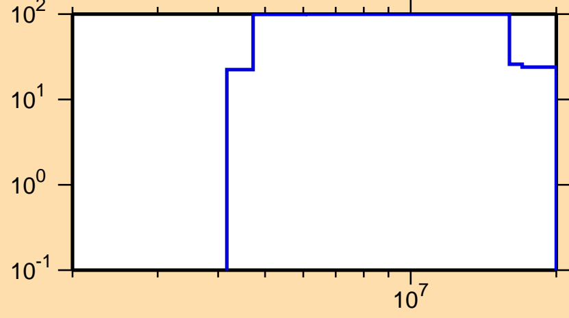
\Delta\sigma/\sigma vs. E for ^{227}\text{At}(n,n\text{cont.})
