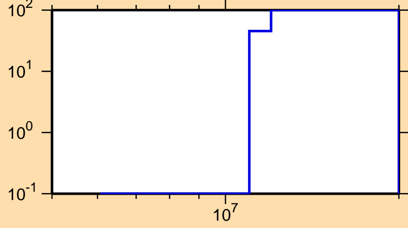
\Delta\sigma/\sigma vs. E for ^{227}\text{At}(n,f)
