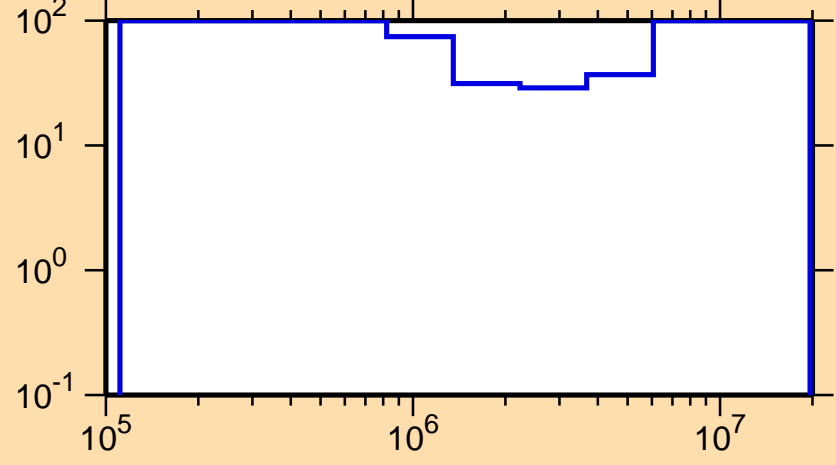
\Delta\sigma/\sigma vs. E for ^{227}\text{At}(n,ncont.)
