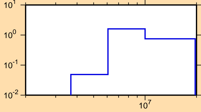
\sigma vs. E for ^{227}\text{At}(n,2n)
