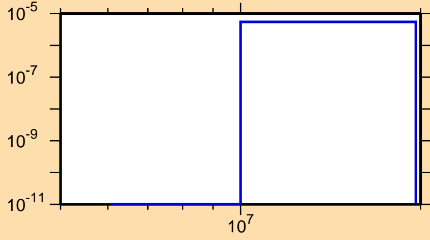
\sigma vs. E for ^{227}\text{At}(n,n\alpha)
