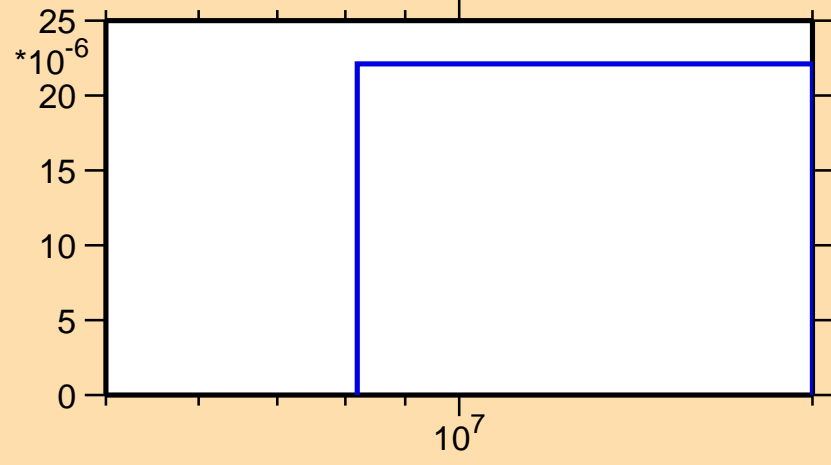
\sigma vs. E for ^{227}\text{At}(n,t)
