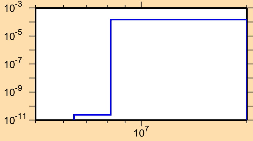
\sigma vs. E for ^{227}\text{At}(n,p)
