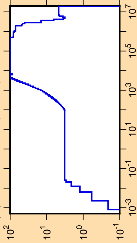
\Delta\mu/\mu vs. E for ^{228}\text{At}(\text{mt251})
