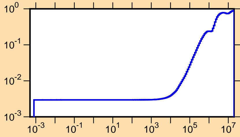
\mu vs. E for ^{228}\text{At}(\text{mt251})
