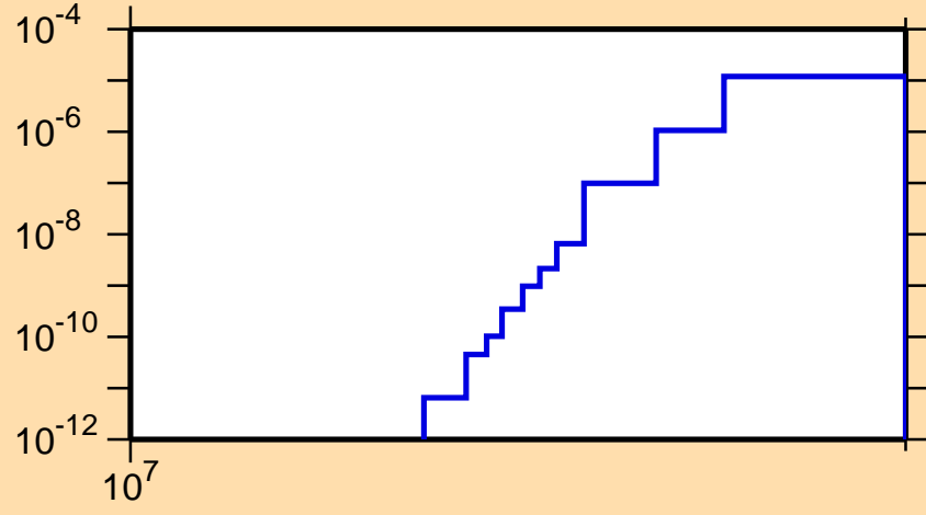
\sigma vs. E for ^{228}\text{At}(n,nd)
