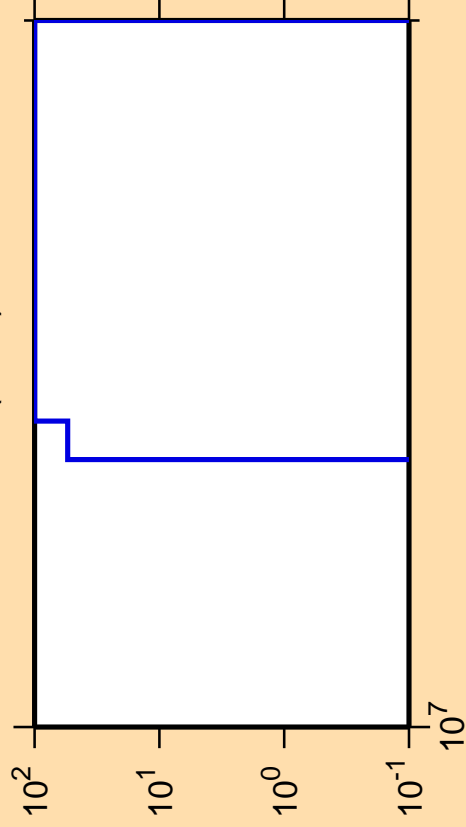
\Delta\sigma/\sigma vs. E for ^{228}\text{At}(n,nd)
