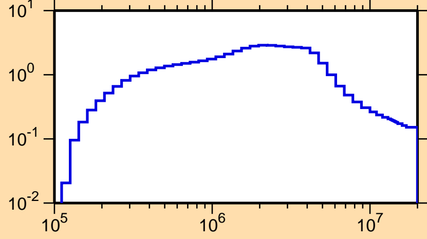
\sigma vs. E for ^{228}\text{At}(n,\text{inel.})
