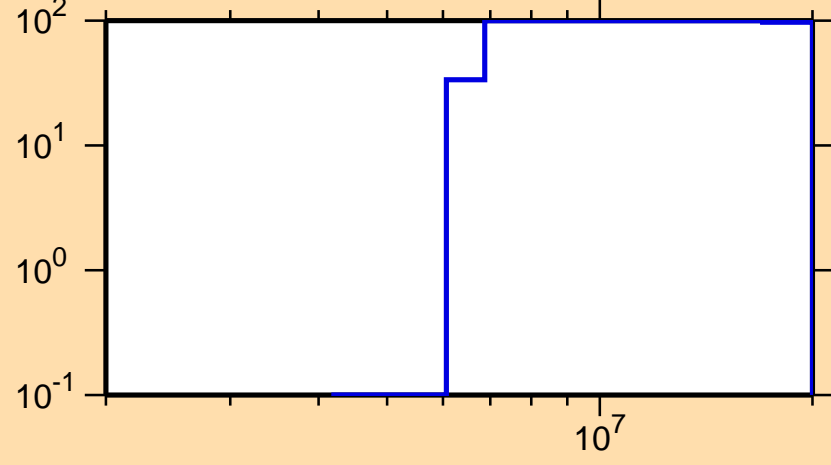
\Delta\sigma/\sigma vs. E for ^{228}\text{At}(n,p)
