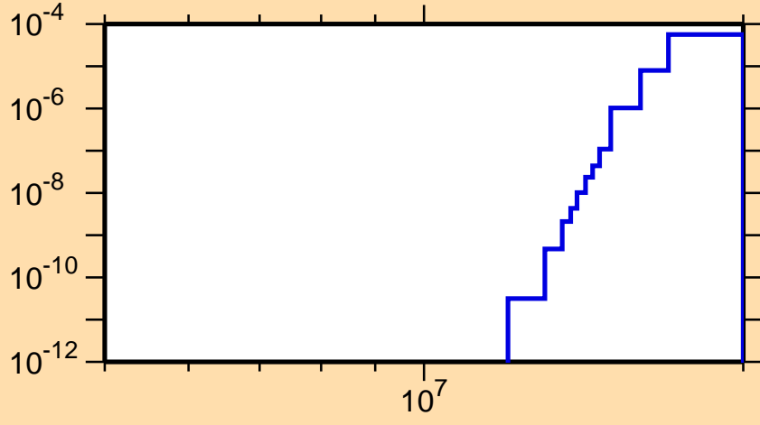
\sigma vs. E for ^{228}\text{At}(n,nt)
