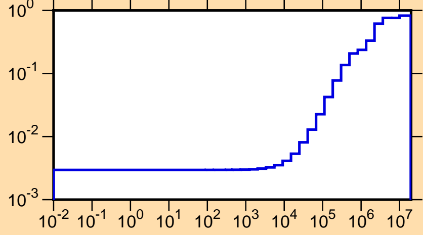
\mu vs. E for ^{228}\text{At}(\text{mt251})
