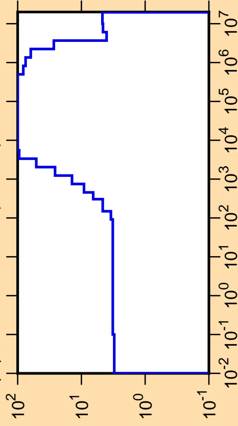
\Delta\mu/\mu vs. E for ^{228}\text{At}(\text{mt251})
