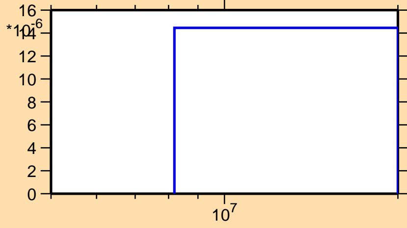
\sigma vs. E for ^{228}\text{At}(n,d)
