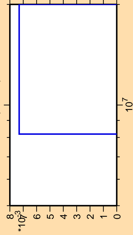
\Delta\sigma/\sigma vs. E for ^{228}\text{At}(\text{mt } 42)
