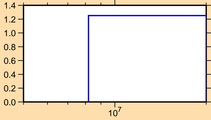
\sigma vs. E for ^{228}\text{At}(n,3n)
