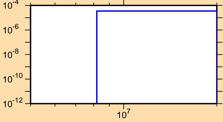
\sigma vs. E for ^{228}\text{At}(n,t)
