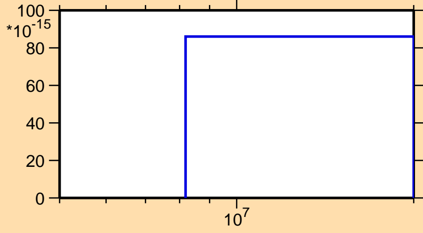
\sigma vs. E for ^{228}\text{At}(n,3n\alpha)
