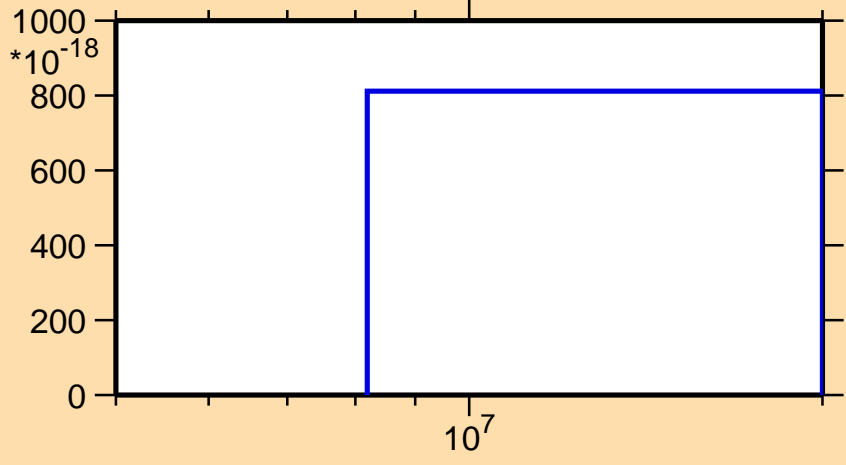
\sigma vs. E for ^{228}\text{At}(\text{mt } 42)
