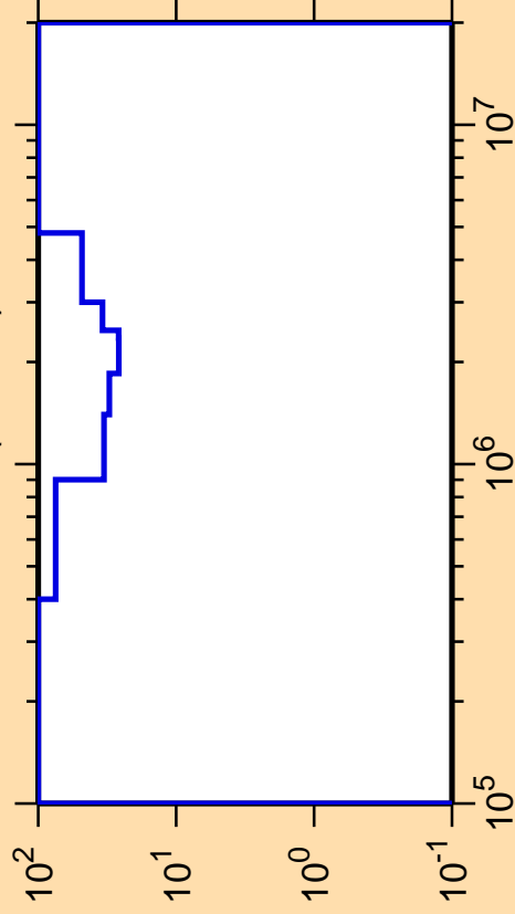
\Delta\sigma/\sigma vs. E for ^{228}\text{At}(n,\text{inel.})
