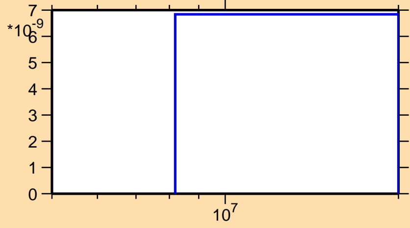
\sigma vs. E for ^{228}\text{At}(n,2np)
