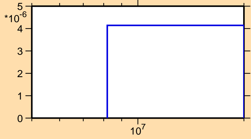
\sigma vs. E for ^{228}\text{At}(n,np)
