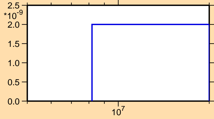
\sigma vs. E for ^{228}\text{At}(n,2n\alpha)
