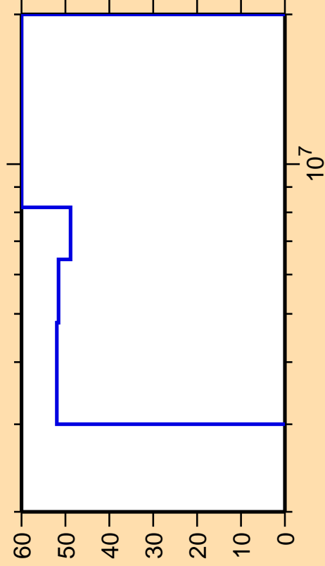
\Delta\sigma/\sigma vs. E for ^{228}\text{At}(n,2n)
