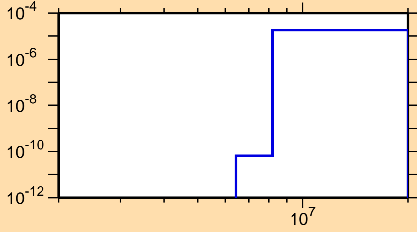
\sigma vs. E for ^{228}\text{At}(n,\alpha)
