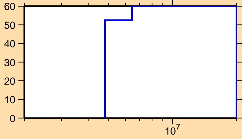
\Delta\sigma/\sigma vs. E for ^{228}\text{At}(n,el.)
