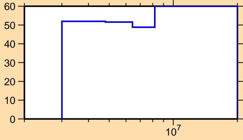
\Delta\sigma/\sigma vs. E for ^{228}\text{At}(n,2n)
