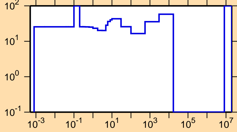
\Delta\sigma/\sigma vs. E for ^{228}\text{At}(n,f)
