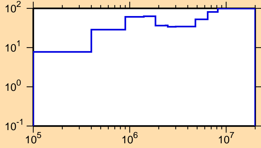
\Delta\sigma/\sigma vs. E for ^{228}\text{At}(n,\text{el.})
