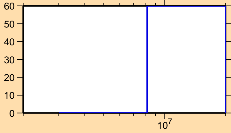
\Delta\sigma/\sigma vs. E for ^{228}\text{At}(n,f)
