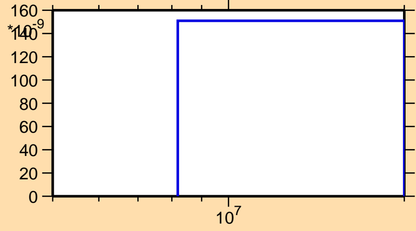
\sigma vs. E for ^{228}\text{At}(n,\text{nd})
