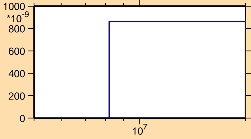
\sigma vs. E for ^{228}\text{At}(n,n\alpha)
