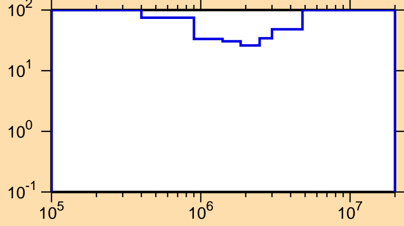
\Delta\sigma/\sigma vs. E for ^{228}\text{At}(n,\text{inel.})
