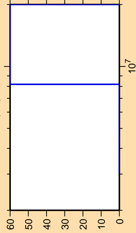
\Delta\sigma/\sigma vs. E for ^{228}\text{At}(n,f)
