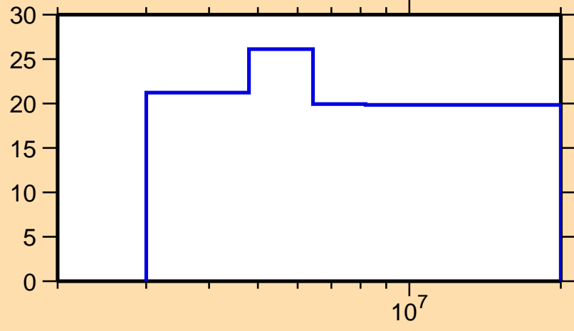
\Delta\sigma/\sigma vs. E for ^{228}\text{At}(n,\text{nonel.})
