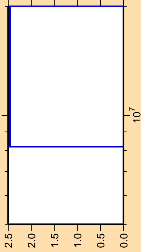
\Delta\sigma/\sigma vs. E for ^{228}\text{At}(\text{mt } 11)
