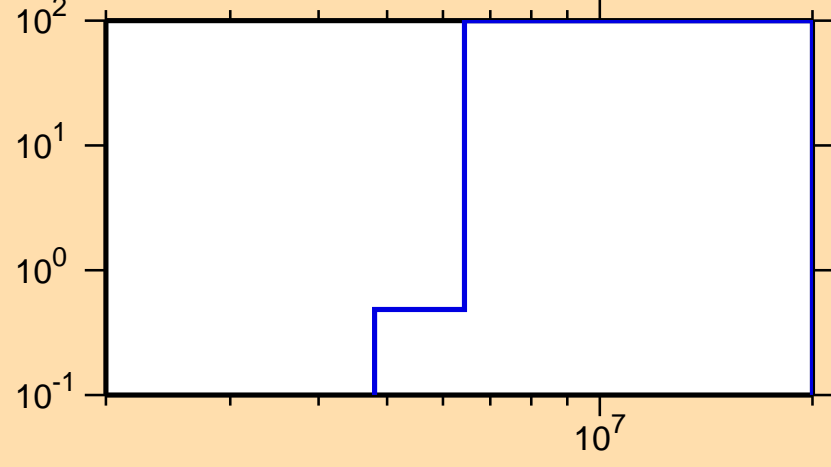
\Delta\sigma/\sigma vs. E for ^{228}\text{At}(n,p)
