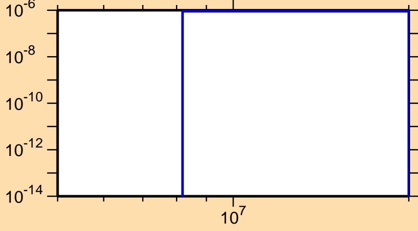
\sigma vs. E for ^{228}\text{At}(n,nt)
