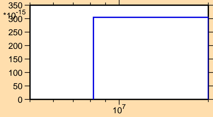
\sigma vs. E for ^{228}\text{At}(\text{mt } 11)
