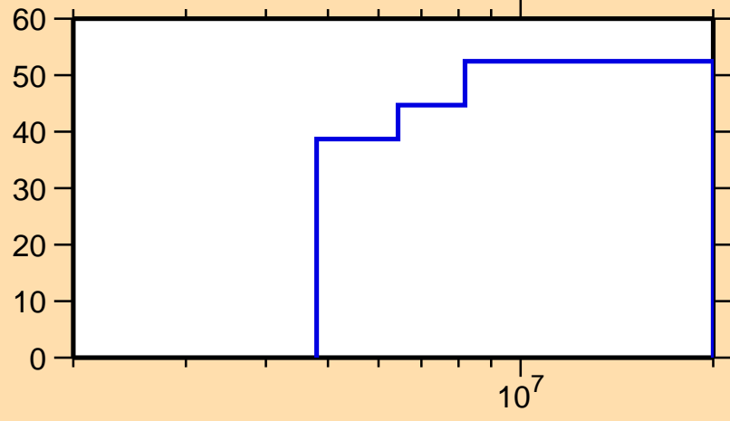
\Delta\sigma/\sigma vs. E for ^{228}\text{At}(n,\text{tot.})
