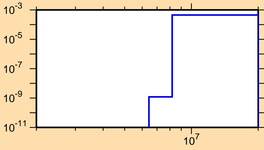
\sigma vs. E for ^{228}\text{At}(n,p)
