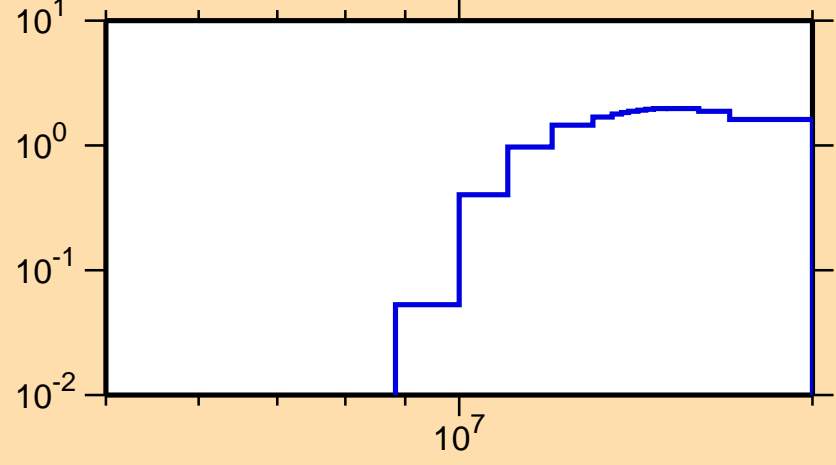
\sigma vs. E for ^{229}\text{At}(n,3n)
