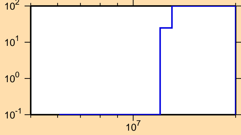
\Delta\sigma/\sigma vs. E for ^{229}\text{At}(n,f)
