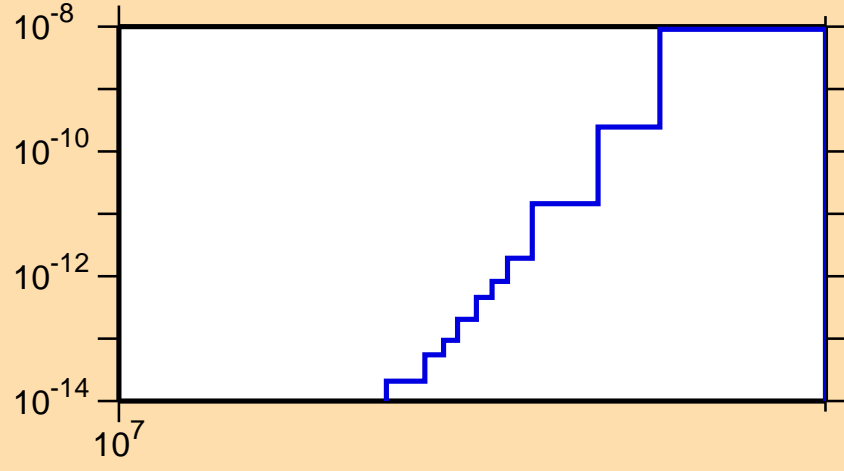
\sigma vs. E for ^{229}\text{At}(n,2n\alpha)
