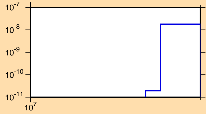
\sigma vs. E for ^{229}\text{At}(n,2np)
