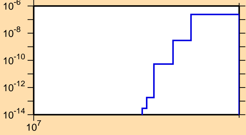
\sigma vs. E for ^{229}\text{At}(n,nd)
