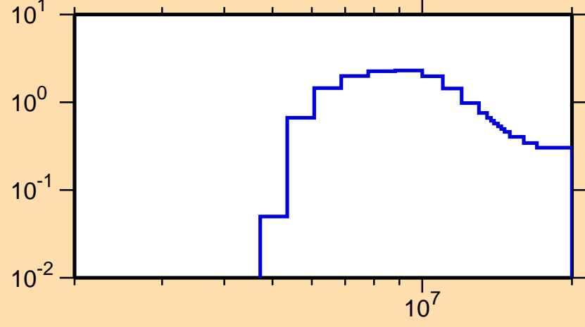
\sigma vs. E for ^{229}\text{At}(n,2n)
