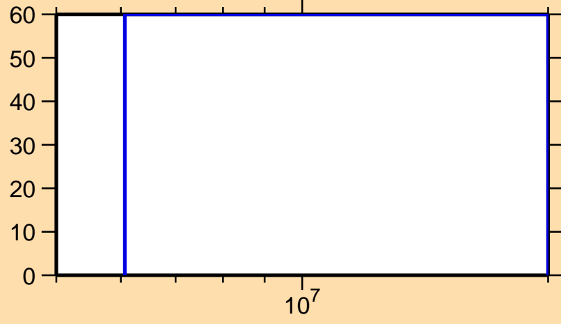
\Delta\sigma/\sigma vs. E for ^{229}\text{At}(n,\text{inel.})
