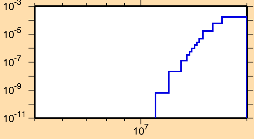
\sigma vs. E for ^{229}\text{At}(n,t)
