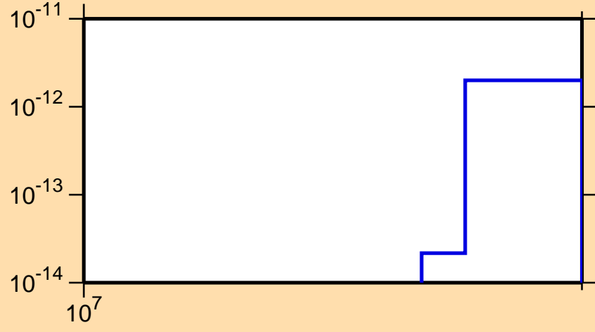
\sigma vs. E for ^{229}\text{At}(n,3n\alpha)
