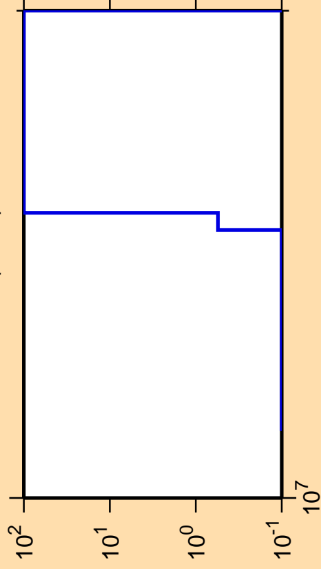
\Delta\sigma/\sigma vs. E for ^{229}\text{At}(n,nd)
