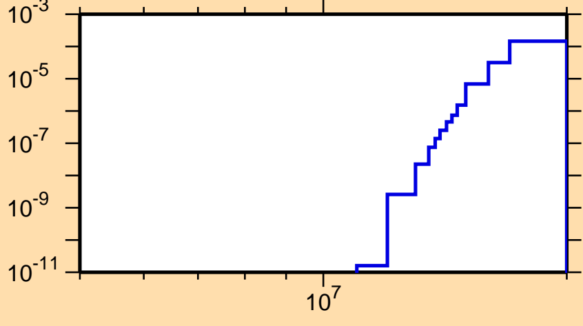
\sigma vs. E for ^{229}\text{At}(n,np)
