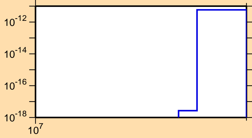
\sigma vs. E for ^{229}\text{At}(\text{mt } 11)
