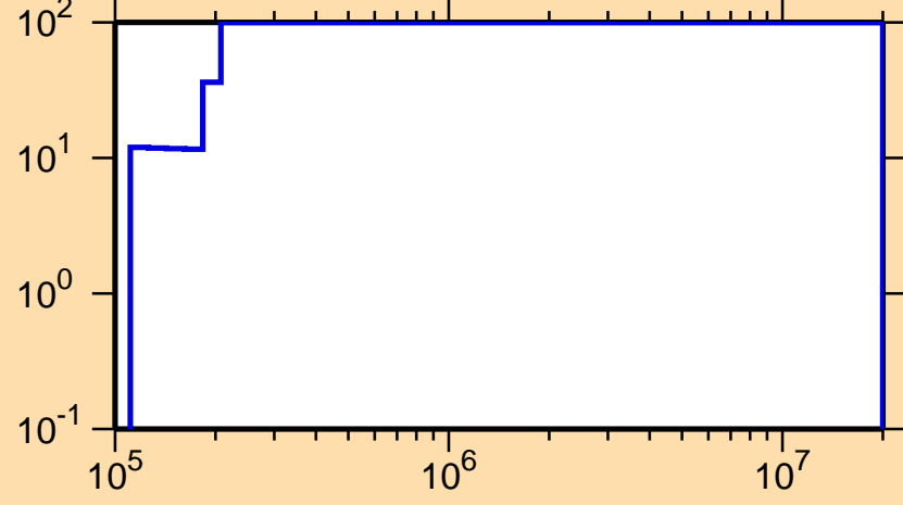
\Delta\sigma/\sigma vs. E for ^{229}\text{At}(n,\text{el.})
