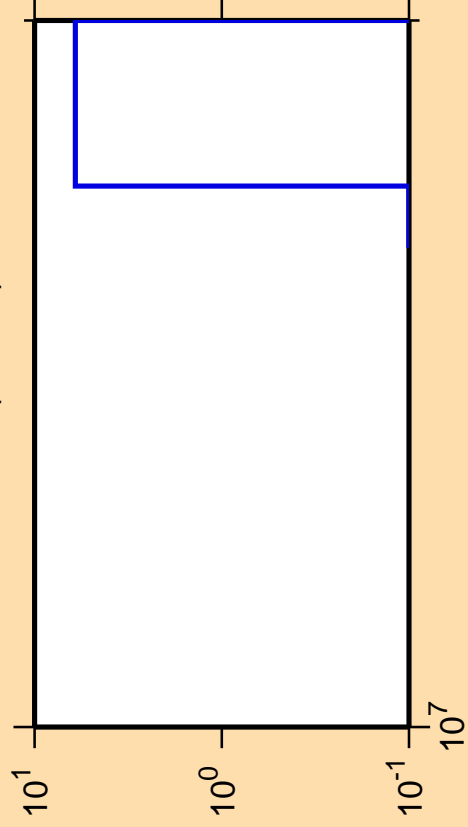
\Delta\sigma/\sigma vs. E for ^{229}\text{At}(n,3n\alpha)
