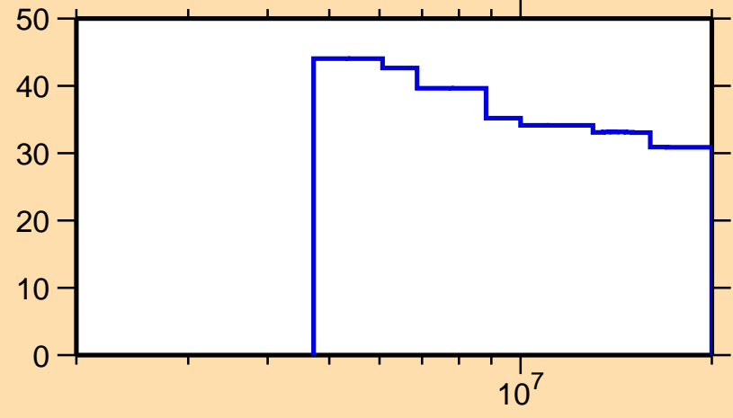
\Delta\sigma/\sigma vs. E for ^{229}\text{At}(n,\text{nonel.})
