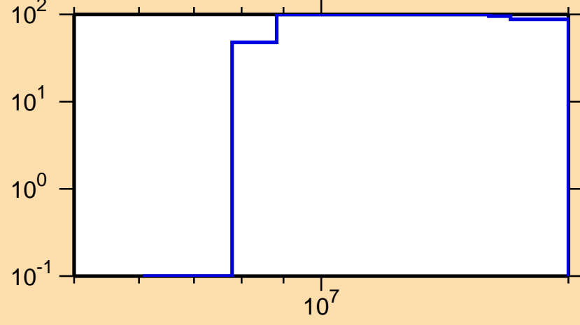
\Delta\sigma/\sigma vs. E for ^{229}\text{At}(n,p)
