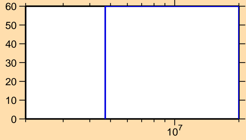
\Delta\sigma/\sigma vs. E for ^{229}\text{At}(n,2n)
