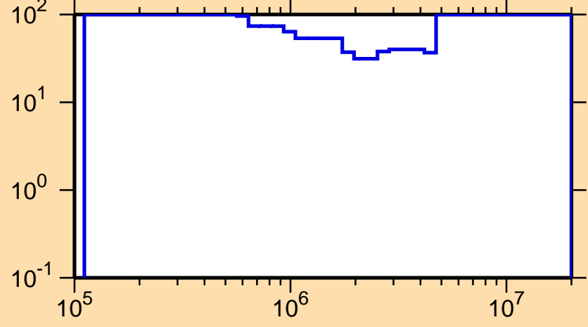
\Delta\sigma/\sigma vs. E for ^{229}\text{At}(n,\text{inel.})
