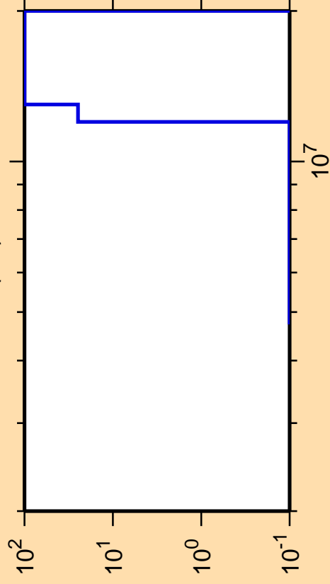
\Delta\sigma/\sigma vs. E for ^{229}\text{At}(n,f)
