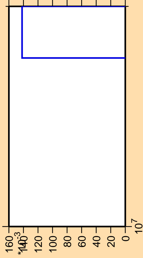
\Delta\sigma/\sigma vs. E for ^{229}\text{At}(\text{mt } 42)
