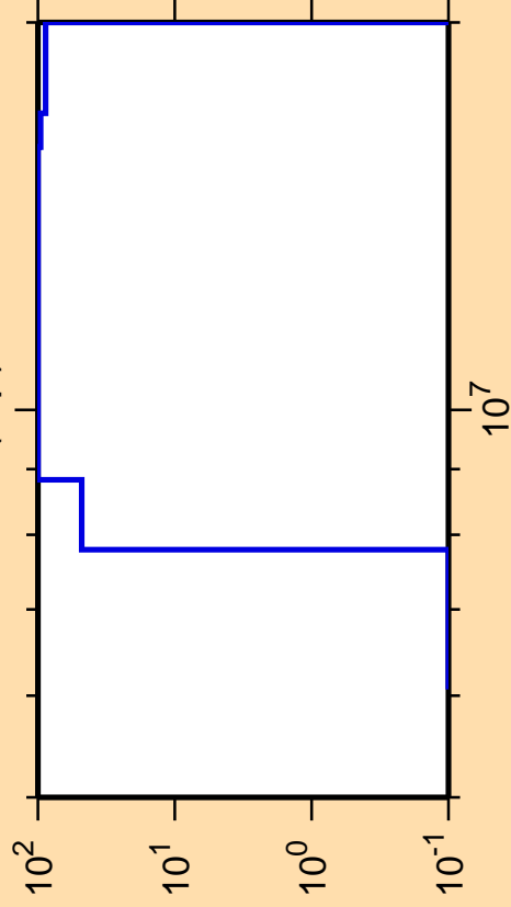
\Delta\sigma/\sigma vs. E for ^{229}\text{At}(n,p)
