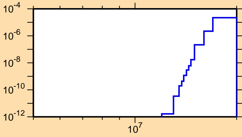
\sigma vs. E for ^{229}\text{At}(n,nt)
