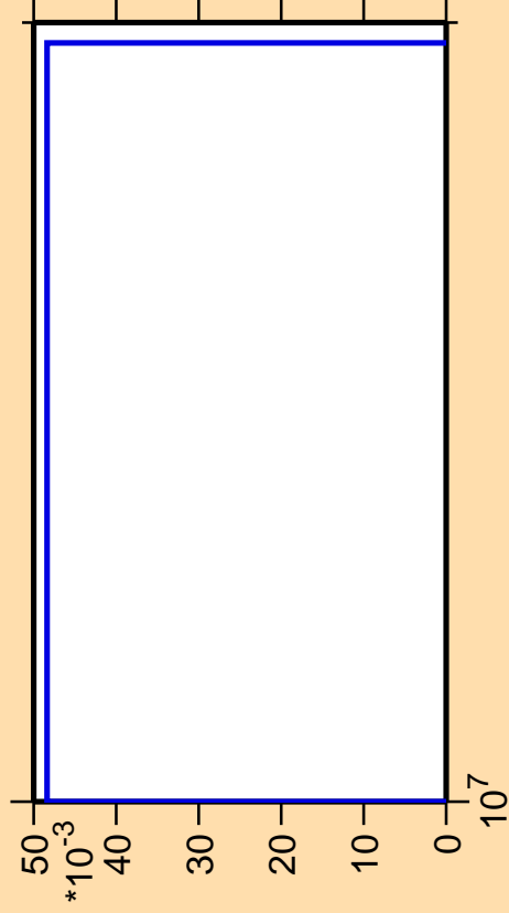
\Delta\sigma/\sigma vs. E for ^{229}\text{At}(n,3n\alpha)
