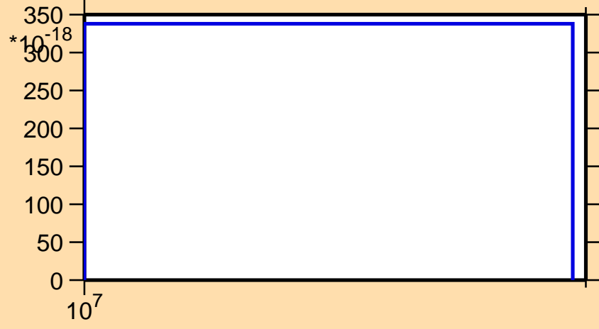
\sigma vs. E for ^{229}\text{At}(\text{mt } 42)
