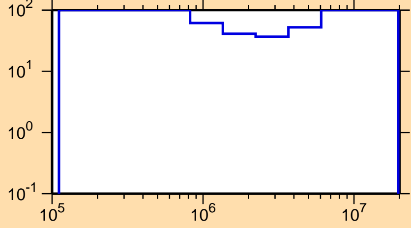
\Delta\sigma/\sigma vs. E for ^{229}\text{At}(n,n\text{cont.})
