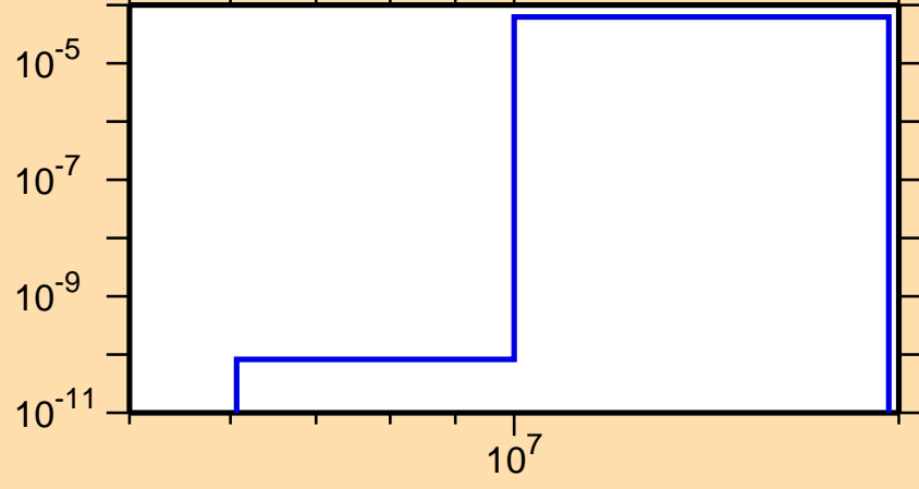
\sigma vs. E for ^{229}\text{At}(n,p)
