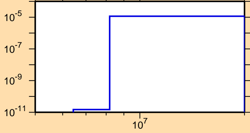
\sigma vs. E for ^{229}\text{At}(n,\alpha)
