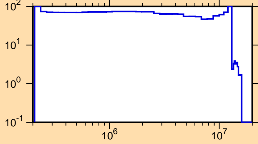
\Delta\sigma/\sigma vs. E for ^{176}\text{Au}(n,n_1)
