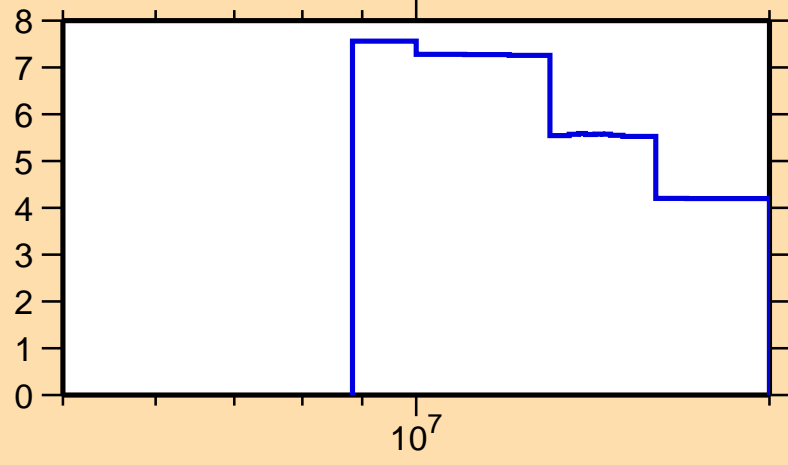
\Delta\sigma/\sigma vs. E for ^{176}\text{Au}(n,\text{el.})
