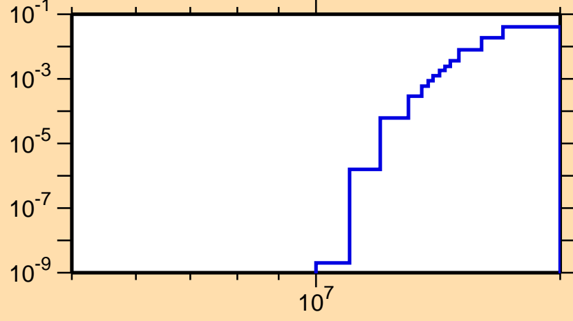
\sigma vs. E for ^{176}\text{Au}(n,2np)
