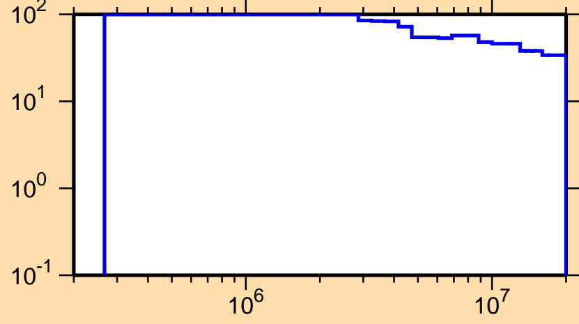
\Delta\sigma/\sigma vs. E for ^{176}\text{Au}(n,n\text{cont.})
