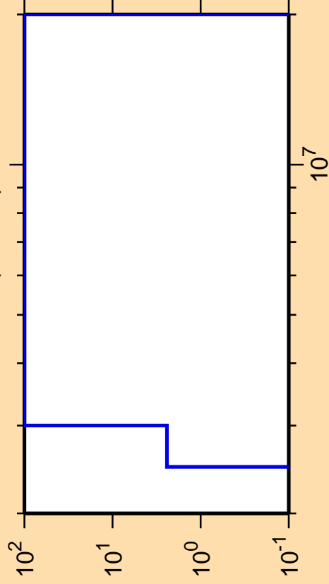
\Delta\sigma/\sigma vs. E for ^{176}\text{Au}(n,\text{He3})
