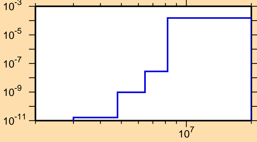
\sigma vs. E for ^{176}\text{Au}(n,\text{He3})
