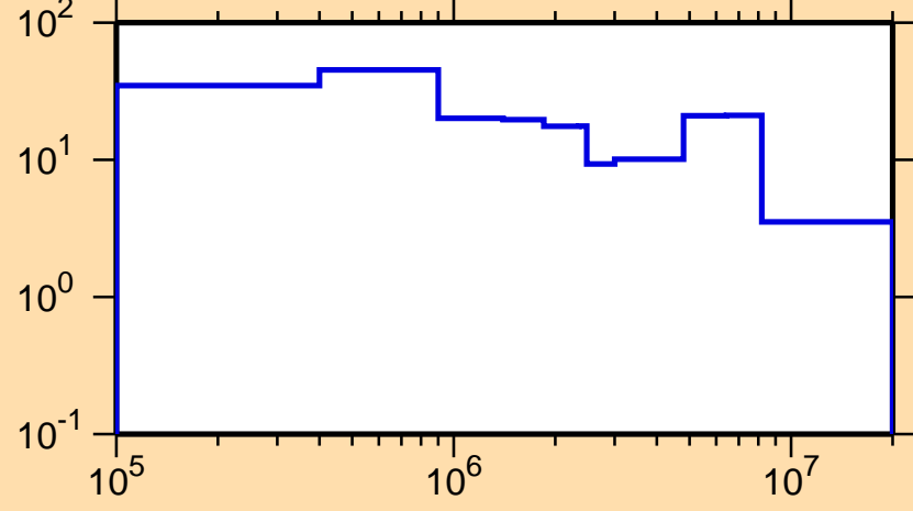
\Delta\sigma/\sigma vs. E for ^{176}\text{Au}(n,\text{el.})
