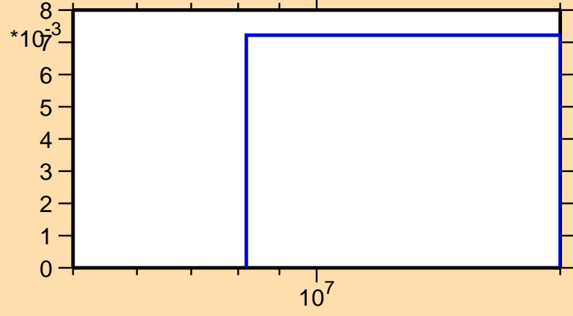
\sigma vs. E for ^{176}\text{Au}(n,2n\alpha)
