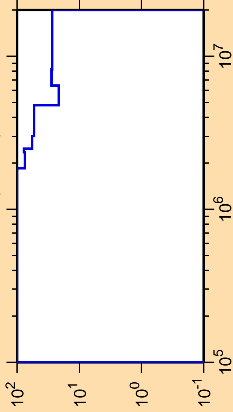
\Delta\sigma/\sigma vs. E for ^{176}\text{Au}(n,\text{inel.})
