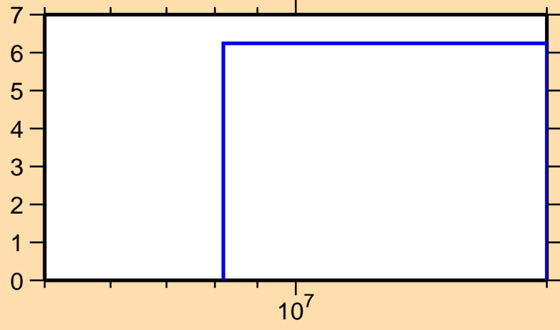
\Delta\sigma/\sigma vs. E for ^{176}\text{Au}(n,\text{nonel.})
