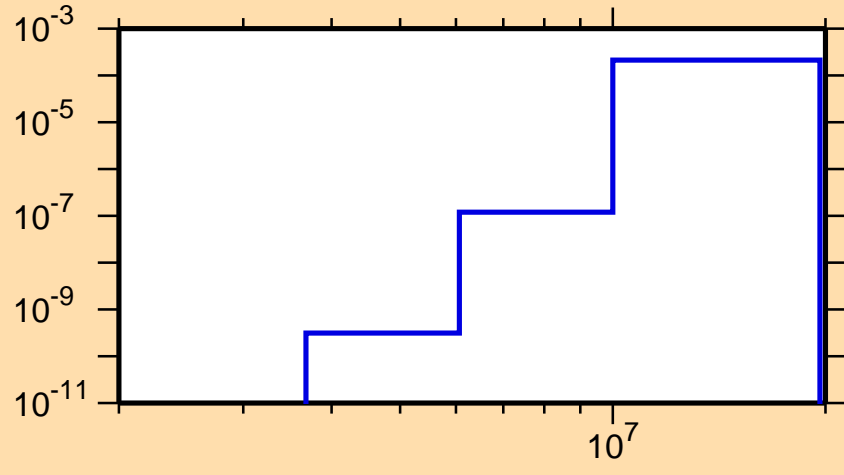
\sigma vs. E for ^{176}\text{Au}(n,\text{He3})
