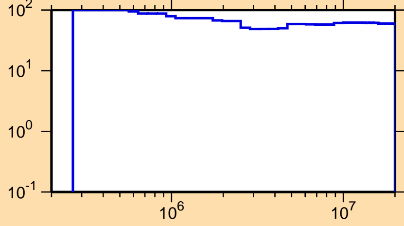
\Delta\sigma/\sigma vs. E for ^{177}\text{Au}(n,n_1)
