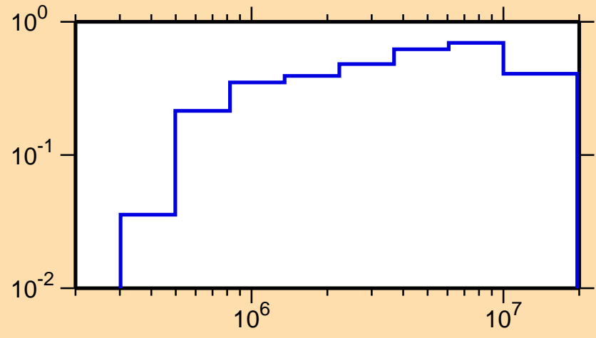
\sigma vs. E for ^{177}\text{Au}(n,\text{inel.})
