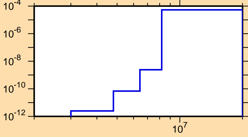
\sigma vs. E for ^{177}\text{Au}(n,\text{He3})
