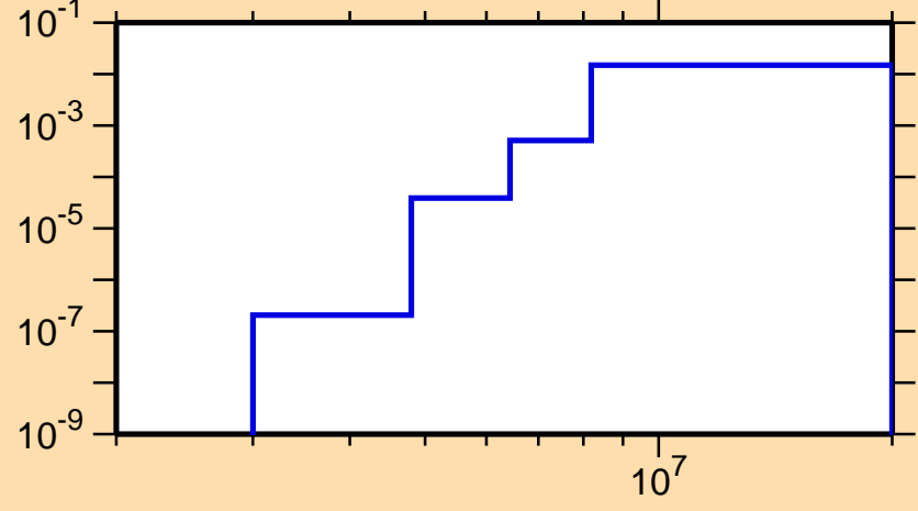
\sigma vs. E for ^{177}\text{Au}(\text{mt } 45)
