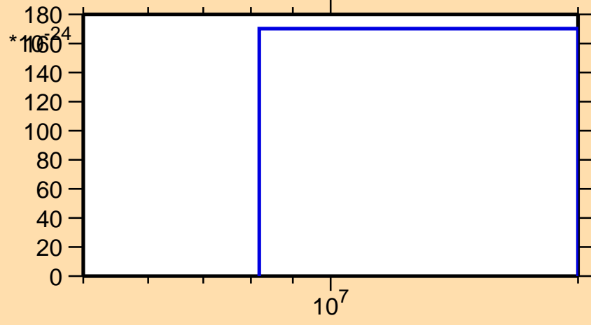
\sigma vs. E for ^{177}\text{Au}(\text{mt } 42)
