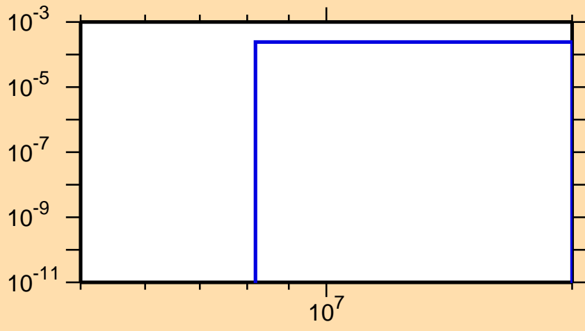
\sigma vs. E for ^{177}\text{Au}(n,t)
