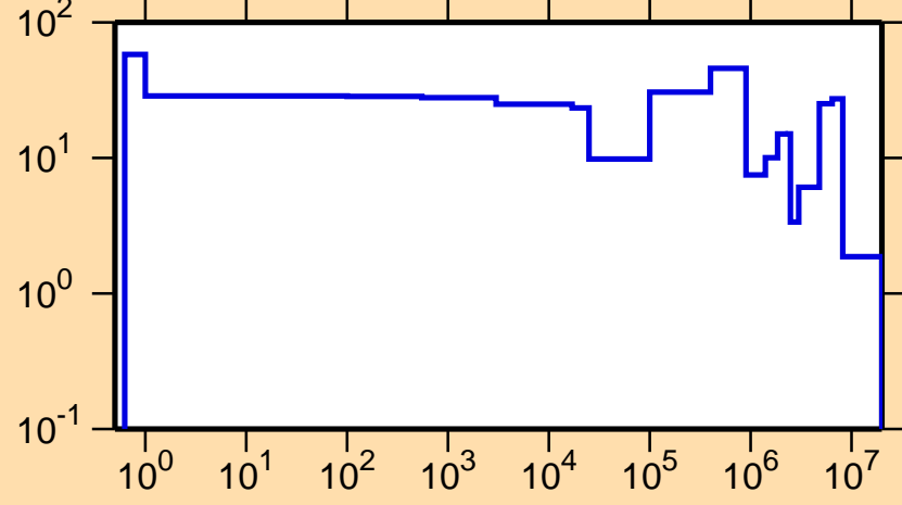
\Delta\sigma/\sigma vs. E for ^{177}\text{Au}(n,\text{el.})
