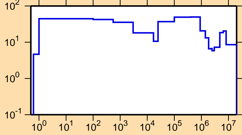
\Delta\sigma/\sigma vs. E for ^{177}\text{Au}(n,\text{tot.})
