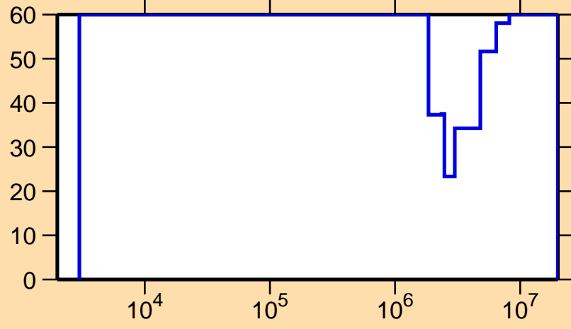
\Delta\sigma/\sigma vs. E for ^{177}\text{Au}(n,ncont.)
