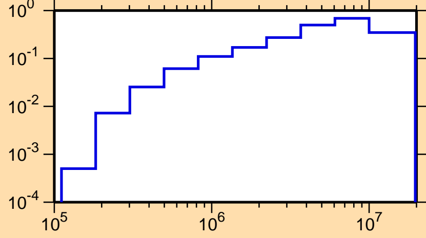
\sigma vs. E for ^{178}\text{Au}(n,\text{inel.})
