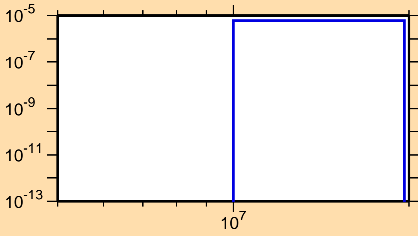
\sigma vs. E for ^{178}\text{Au}(n,\text{nd})
