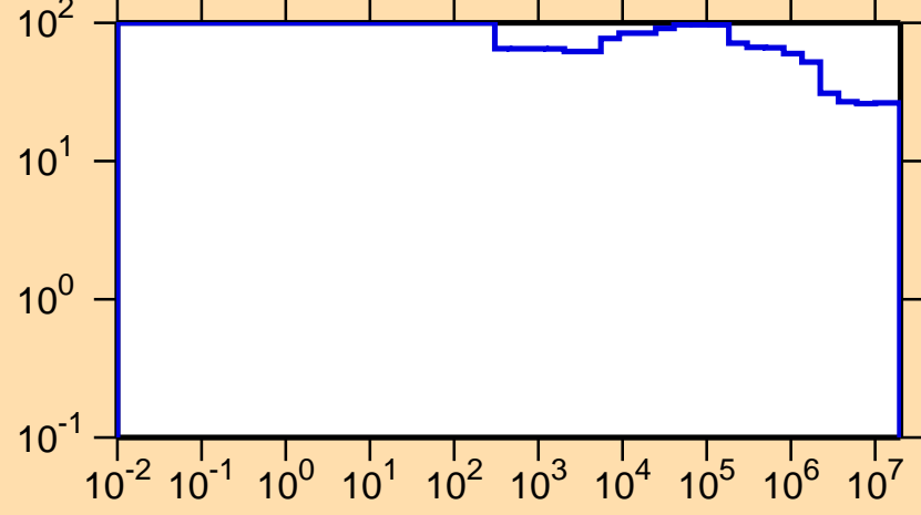
\Delta\sigma/\sigma vs. E for ^{178}\text{Au}(n,\text{nonel.})
