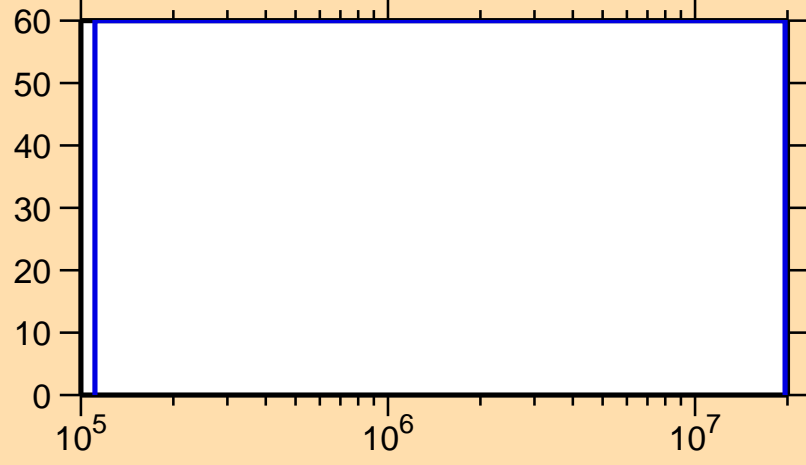
\Delta\sigma/\sigma vs. E for ^{178}\text{Au}(n,ncont.)
