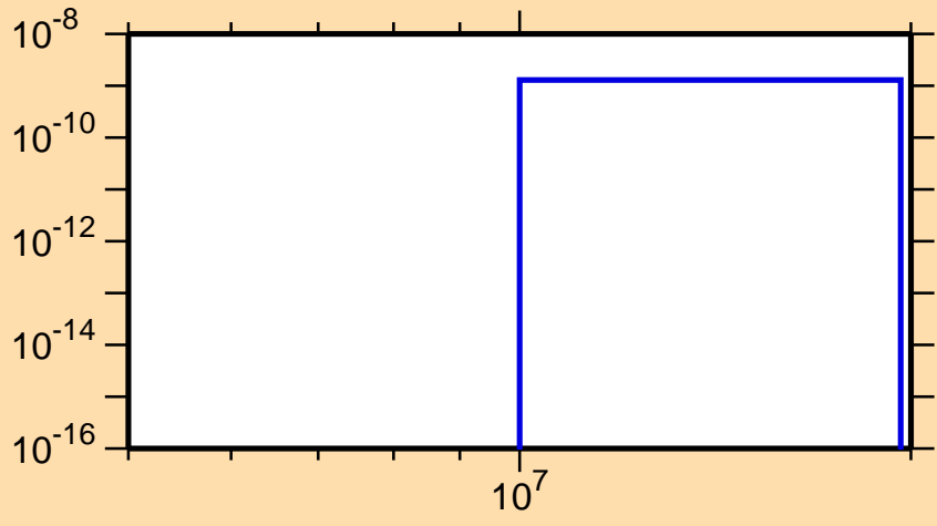
\sigma vs. E for ^{178}\text{Au}(\text{mt } 34)
