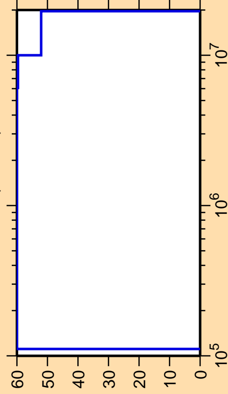
\Delta\sigma/\sigma vs. E for ^{178}\text{Au}(n,\text{inel.})
