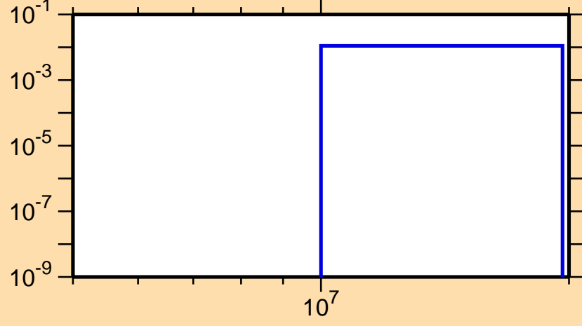
\sigma vs. E for ^{178}\text{Au}(n,2np)
