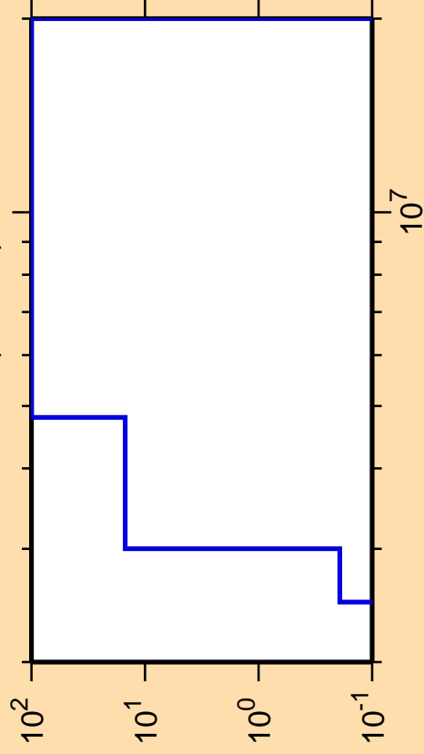
\Delta\sigma/\sigma vs. E for ^{178}\text{Au}(n,\text{He3})
