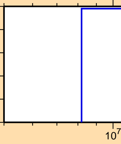
\sigma vs. E for ^{178}\text{Au}(n,\text{nd})
