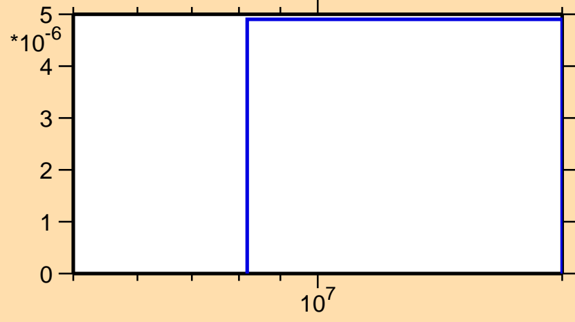
\sigma vs. E for ^{178}\text{Au}(n,\text{nd})
