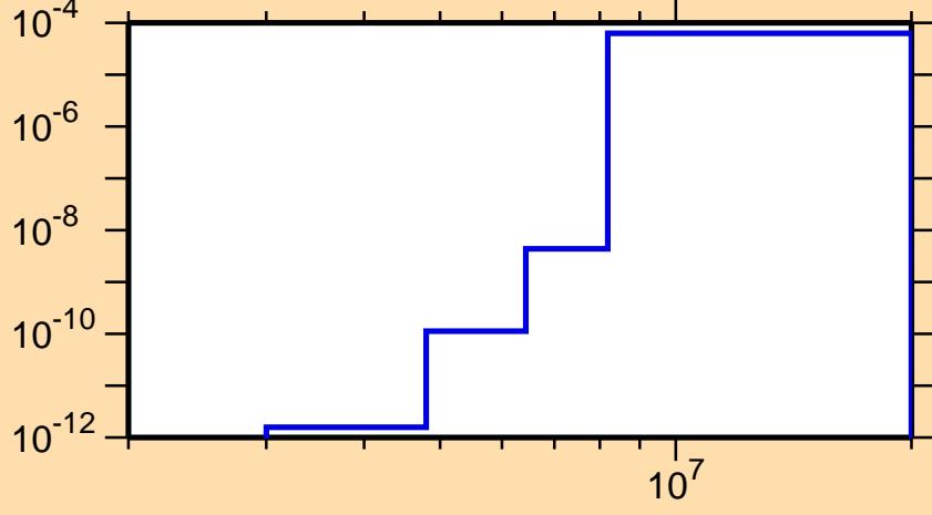
\sigma vs. E for ^{178}\text{Au}(n,\text{He3})
