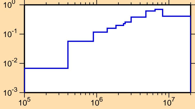
\sigma vs. E for ^{178}\text{Au}(n,\text{inel.})
