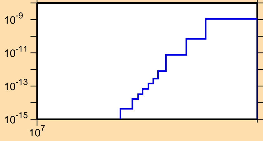
\sigma vs. E for ^{179}\text{Au}(\text{mt } 34)
