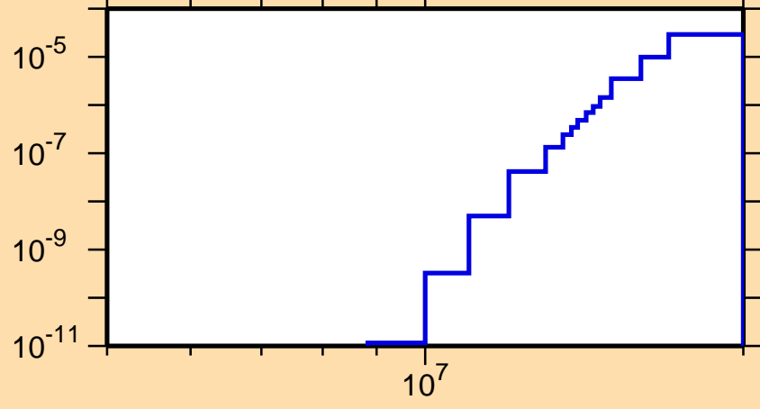
\sigma vs. E for ^{179}\text{Au}(n,\text{pd})
