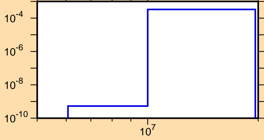
\sigma vs. E for ^{179}\text{Au}(n,t)
