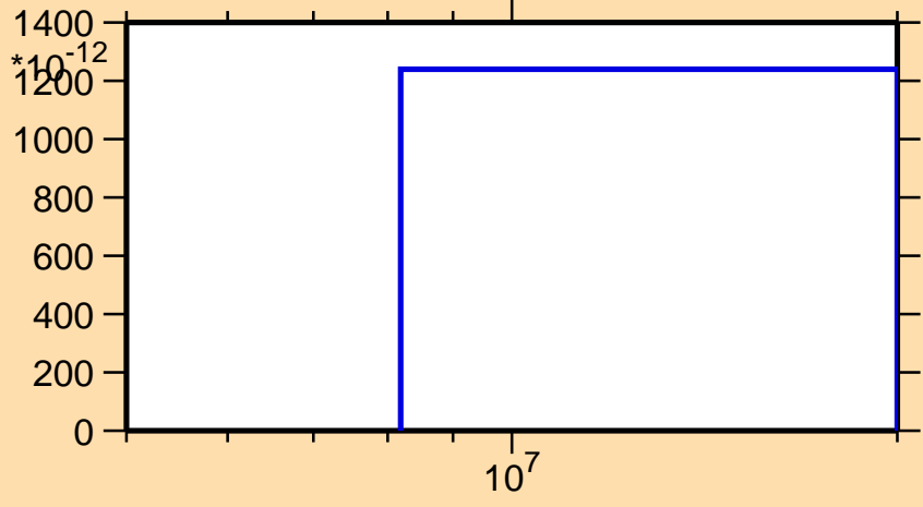
\sigma vs. E for ^{179}\text{Au}(n,\text{pt})
