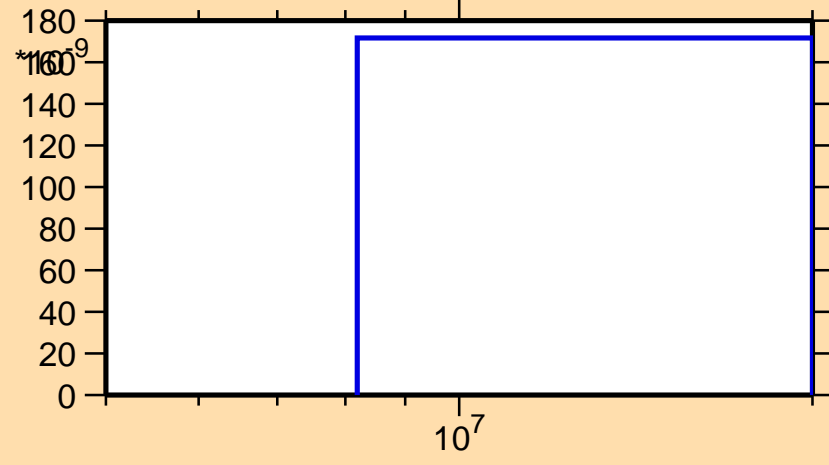
\sigma vs. E for ^{179}\text{Au}(n,\text{nd})
