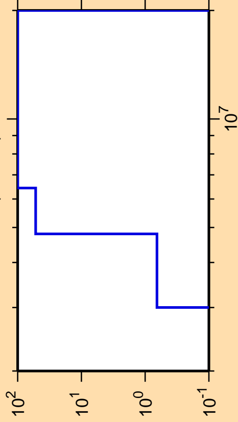
\Delta\sigma/\sigma vs. E for ^{179}\text{Au}(n,\text{He3})
