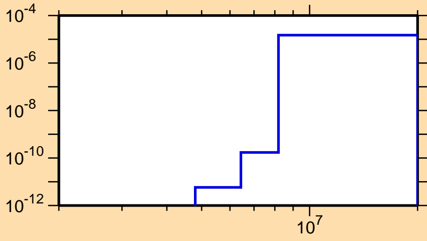
\sigma vs. E for ^{179}\text{Au}(n,\text{He3})
