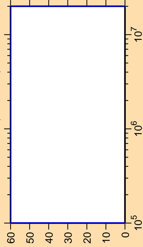
\Delta\sigma/\sigma vs. E for ^{179}\text{Au}(n,\text{ncont.})
