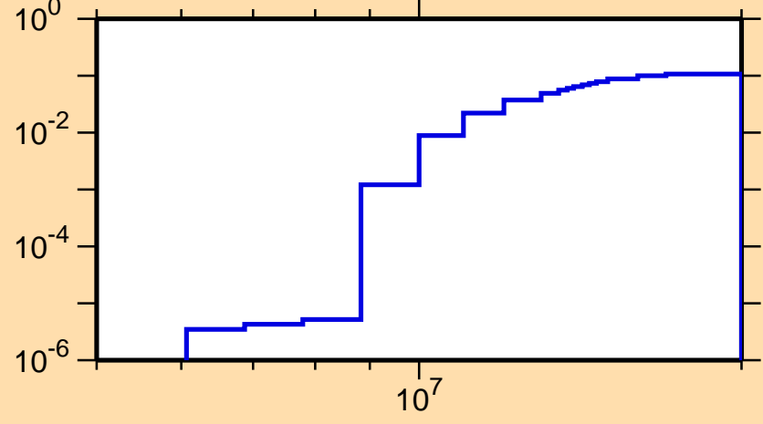
\sigma vs. E for ^{180}\text{Au}(n,2n\alpha)
