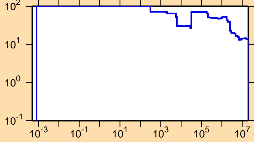
\Delta\sigma/\sigma vs. E for ^{180}\text{Au}(n,\text{nonel.})
