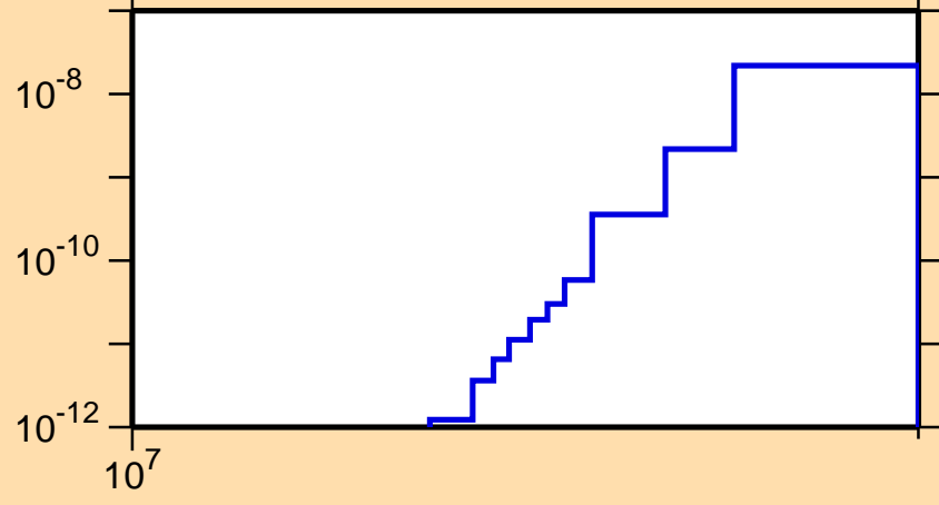
\sigma vs. E for ^{180}\text{Au}(\text{mt } 34)
