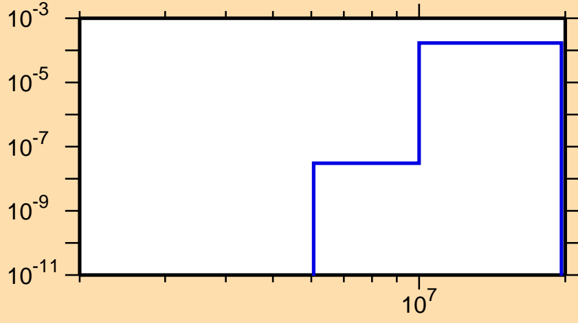
\sigma vs. E for ^{180}\text{Au}(\text{mt } 45)
