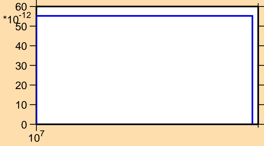
\sigma vs. E for ^{180}\text{Au}(n,3n)
