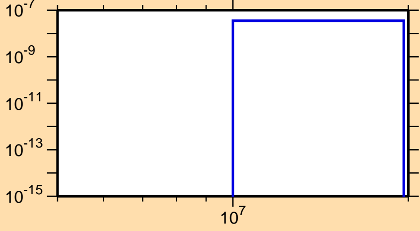
\sigma vs. E for ^{180}\text{Au}(n,\text{pt})
