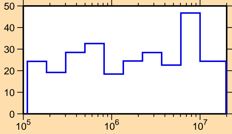
\Delta\sigma/\sigma vs. E for ^{180}\text{Au}(n,el.)
