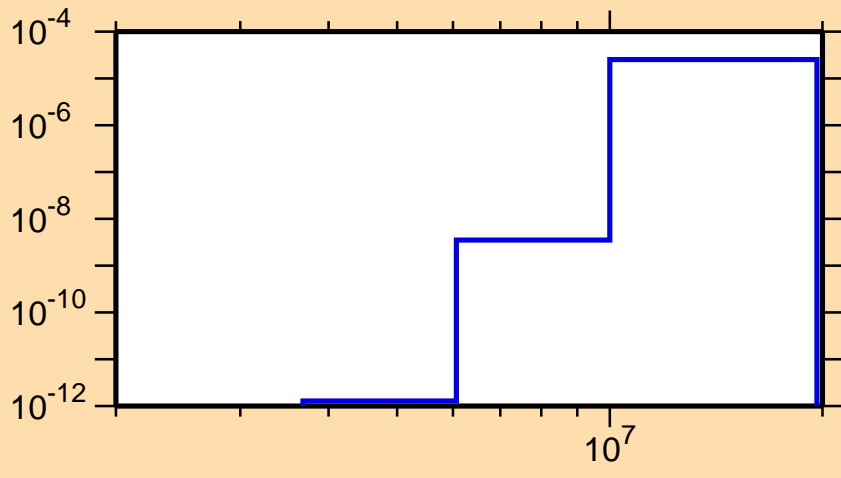
\sigma vs. E for ^{180}\text{Au}(n,\text{He3})
