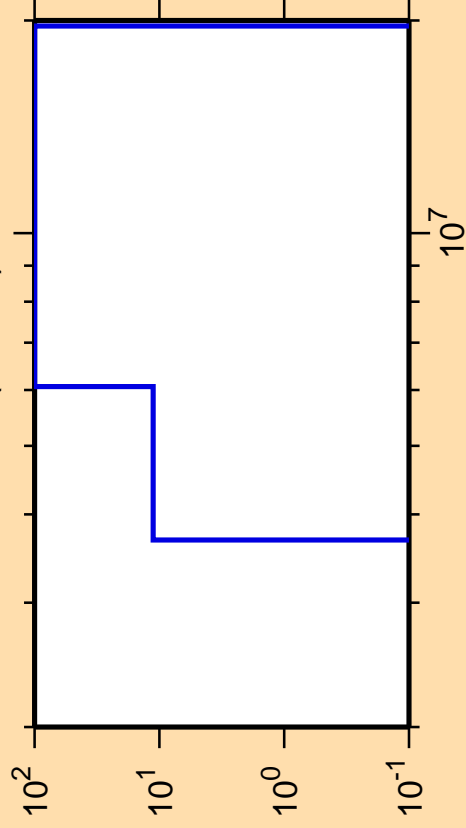
\Delta\sigma/\sigma vs. E for ^{180}\text{Au}(n,\text{He3})
