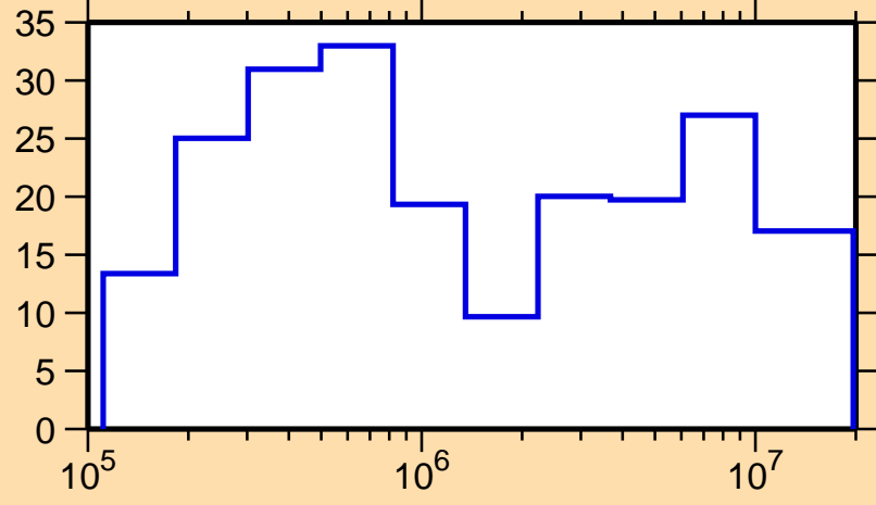
\Delta\sigma/\sigma vs. E for ^{180}\text{Au}(n,tot.)
