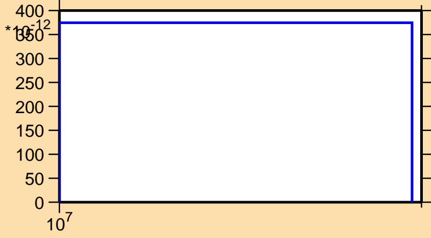
\sigma vs. E for ^{180}\text{Au}(\text{mt } 34)
