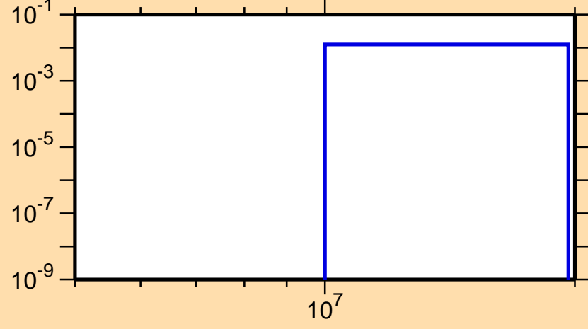
\sigma vs. E for ^{180}\text{Au}(n,2np)
