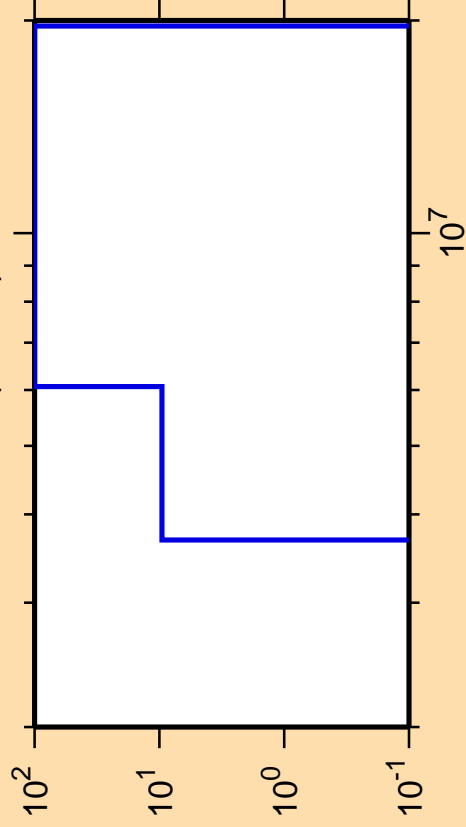
\Delta\sigma/\sigma vs. E for ^{180}\text{Au}(\text{mt } 45)
