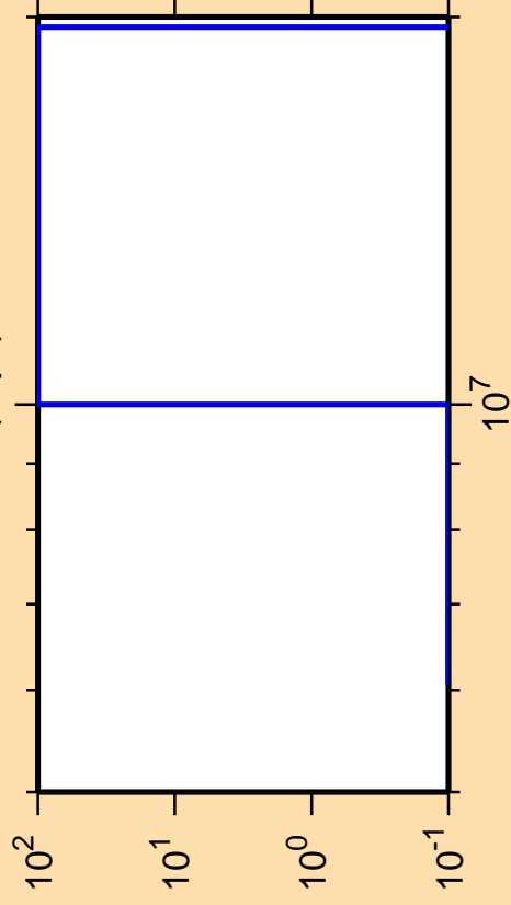
\Delta\sigma/\sigma vs. E for ^{180}\text{Au}(n,\text{pt})
