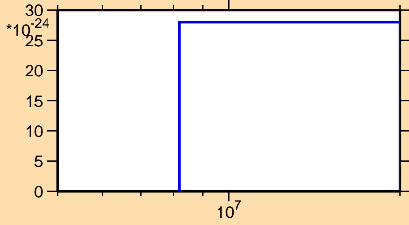
\sigma vs. E for ^{180}\text{Au}(\text{mt } 42)
