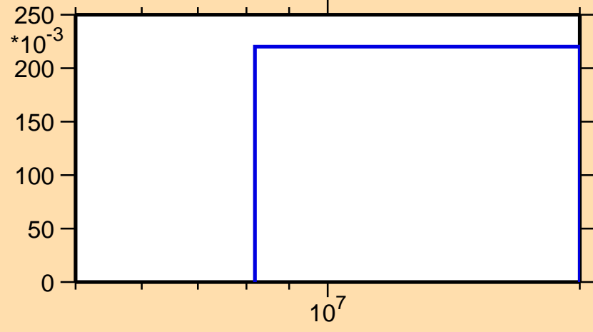
\sigma vs. E for ^{180}\text{Au}(n,2n)
