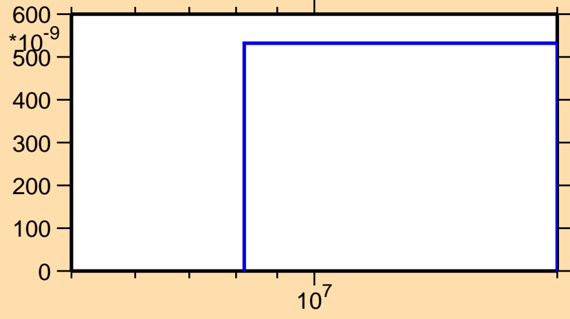
\sigma vs. E for ^{180}\text{Au}(n,\text{pd})
