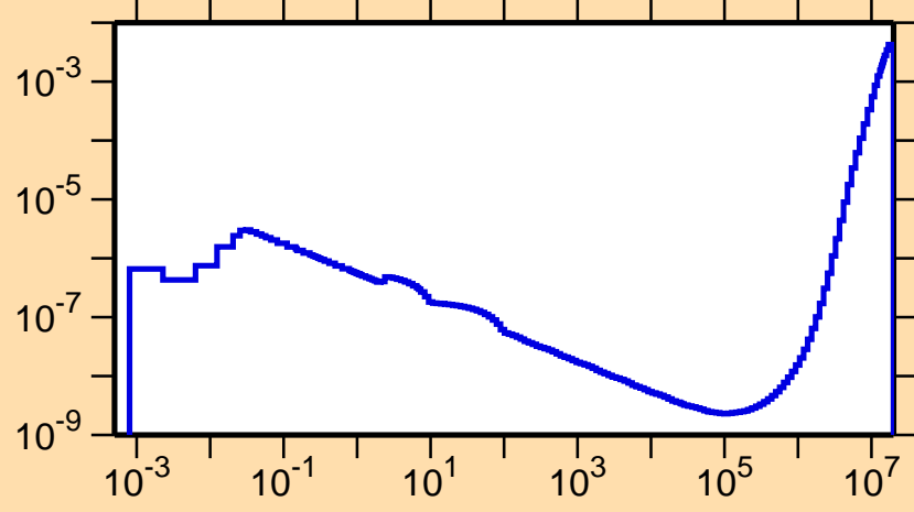
\sigma vs. E for ^{181}\text{Au}(n,p\alpha)
