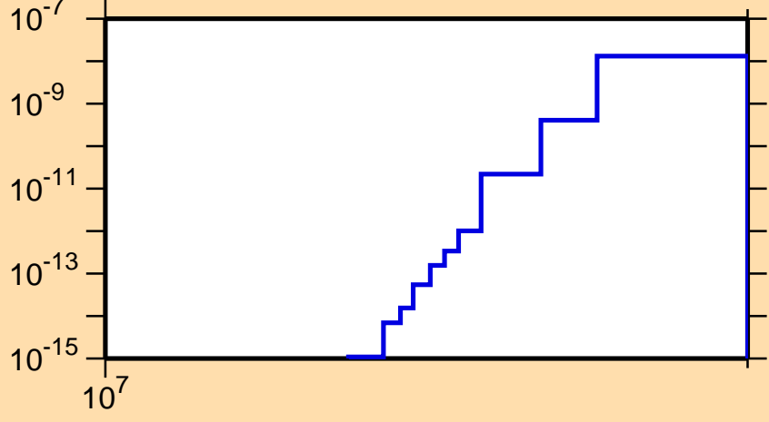
\sigma vs. E for ^{181}\text{Au}(n,pt)
