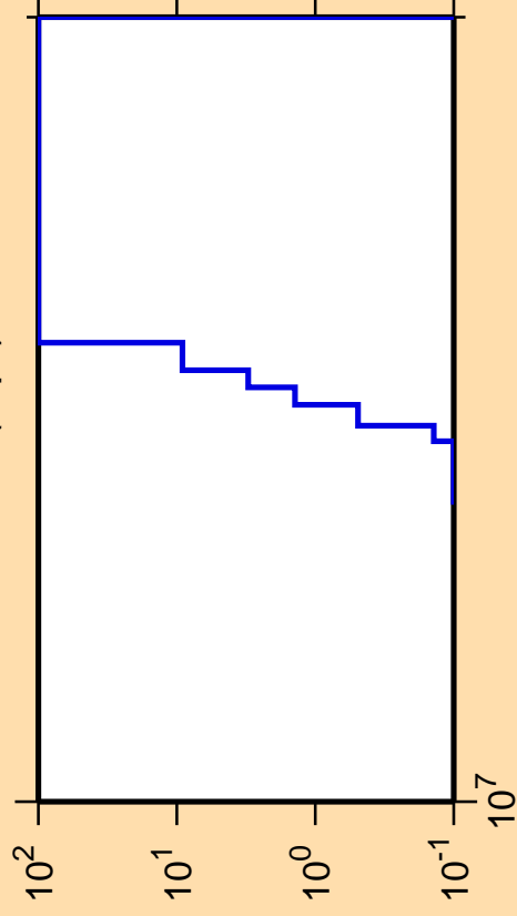
\Delta\sigma/\sigma vs. E for ^{181}\text{Au}(n,pt)
