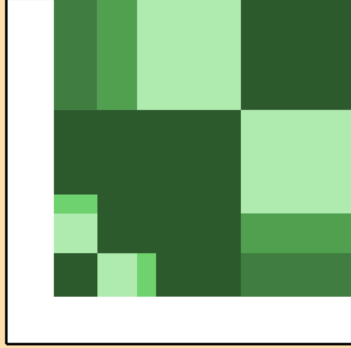
\sigma vs. E for ^{181}\text{Au}(n,2np)
