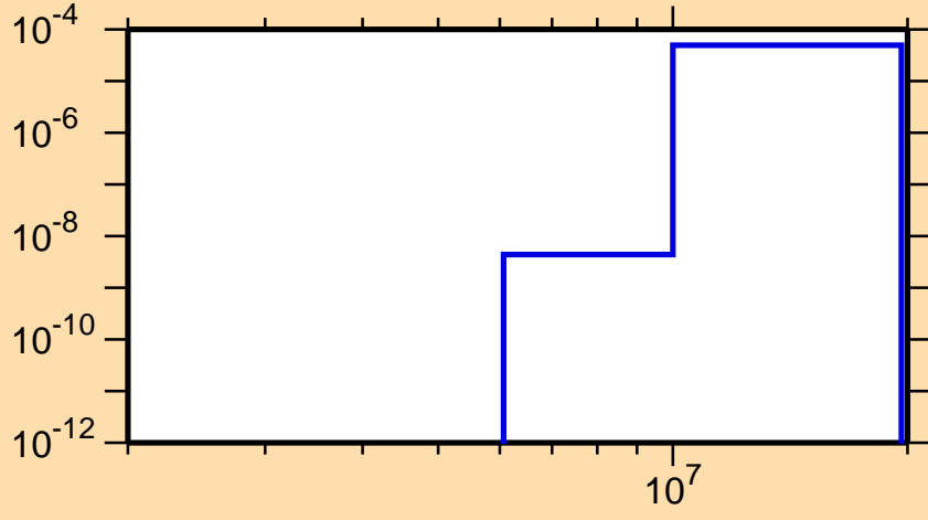
\sigma vs. E for ^{181}\text{Au}(\text{mt } 45)
