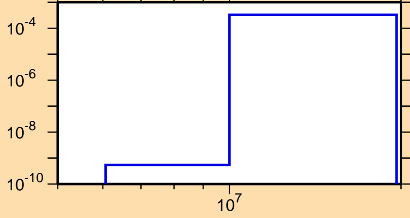
\sigma vs. E for ^{181}\text{Au}(n,t)
