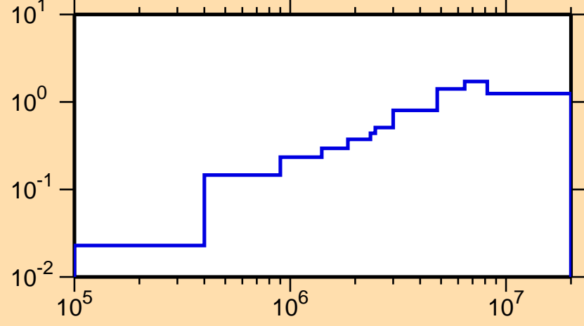
\sigma vs. E for ^{181}\text{Au}(n,\text{inel.})
