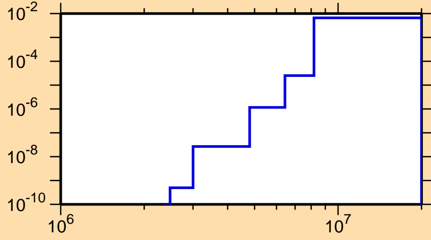
\sigma vs. E for ^{181}\text{Au}(n,d)
