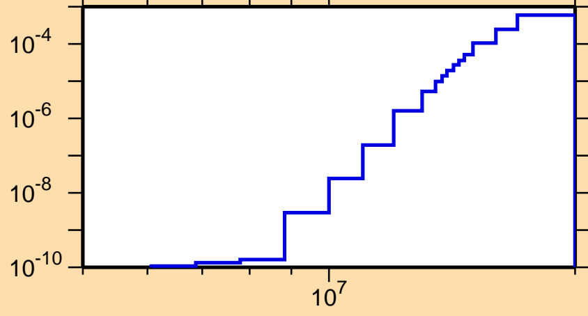
\sigma vs. E for ^{182}\text{Au}(n,2n\alpha)
