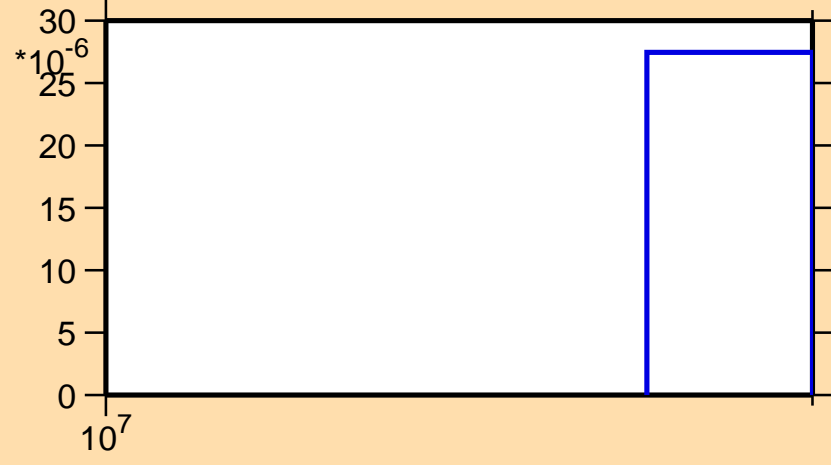
\sigma vs. E for ^{182}\text{Au}(n,3n)
