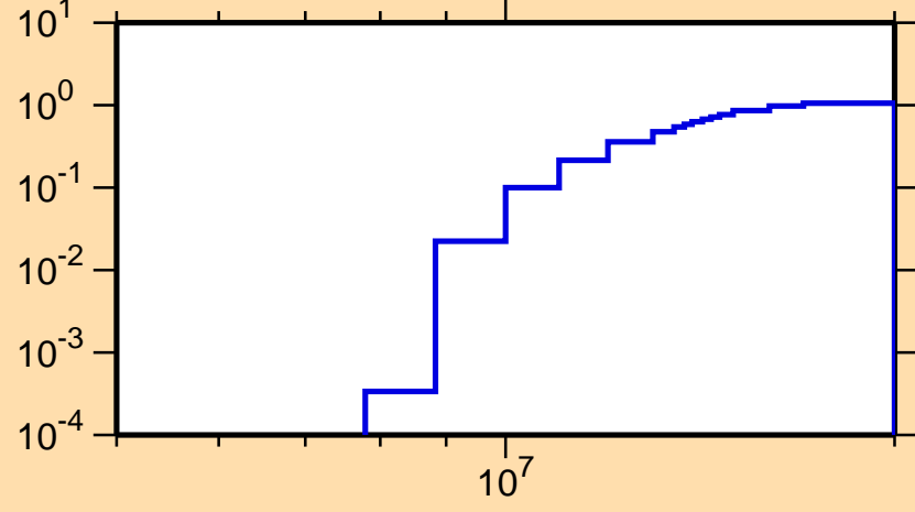
\sigma vs. E for ^{182}\text{Au}(n,2n)
