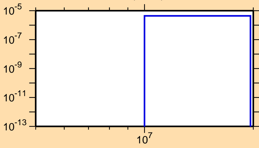
\sigma vs. E for ^{182}\text{Au}(n,\text{nd})
