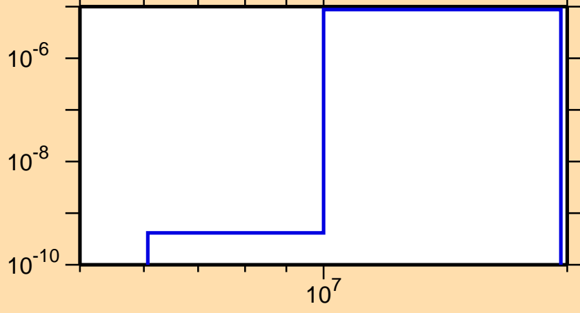
\sigma vs. E for ^{182}\text{Au}(n,\text{He3})
