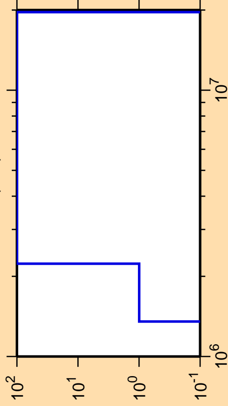
\Delta\sigma/\sigma vs. E for ^{182}\text{Au}(n,d)
