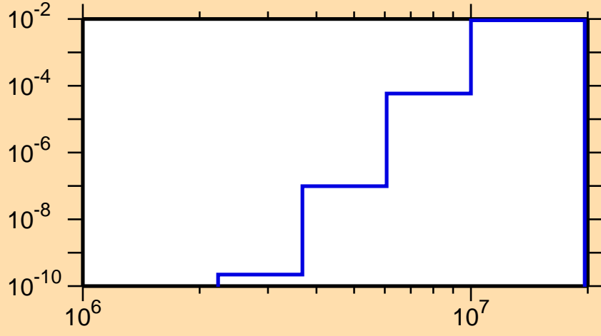
\sigma vs. E for ^{182}\text{Au}(n,d)
