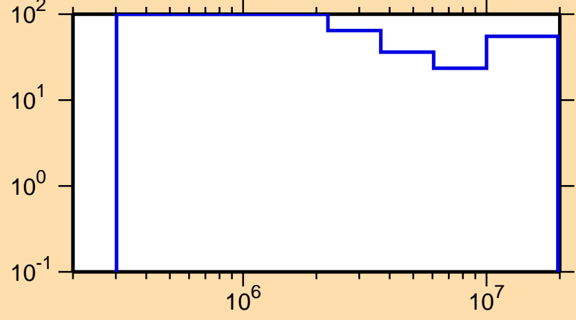
\Delta\sigma/\sigma vs. E for ^{182}\text{Au}(n,ncont.)
