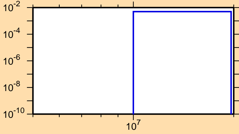
\sigma vs. E for ^{182}\text{Au}(n,2np)
