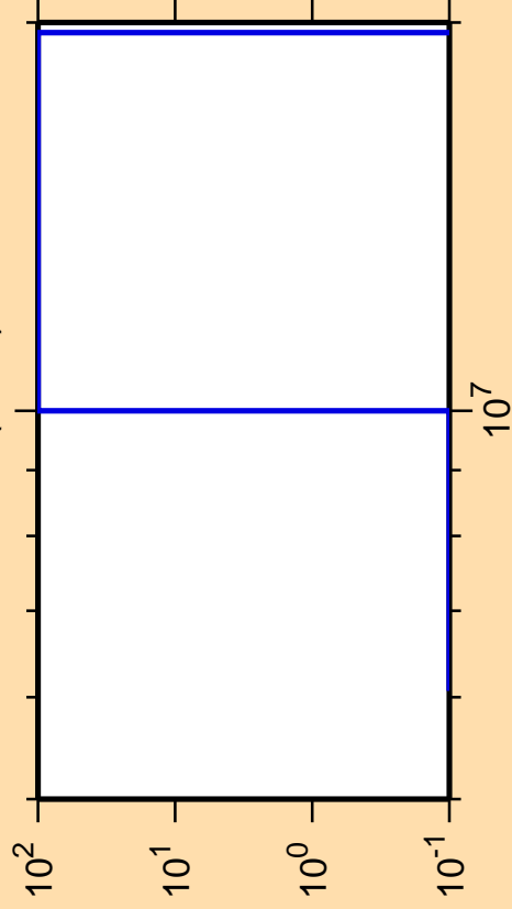
\Delta\sigma/\sigma vs. E for ^{182}\text{Au}(n,\text{nd})
