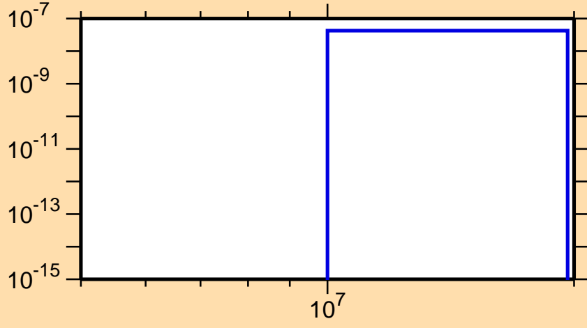
\sigma vs. E for ^{182}\text{Au}(n,\text{pd})
