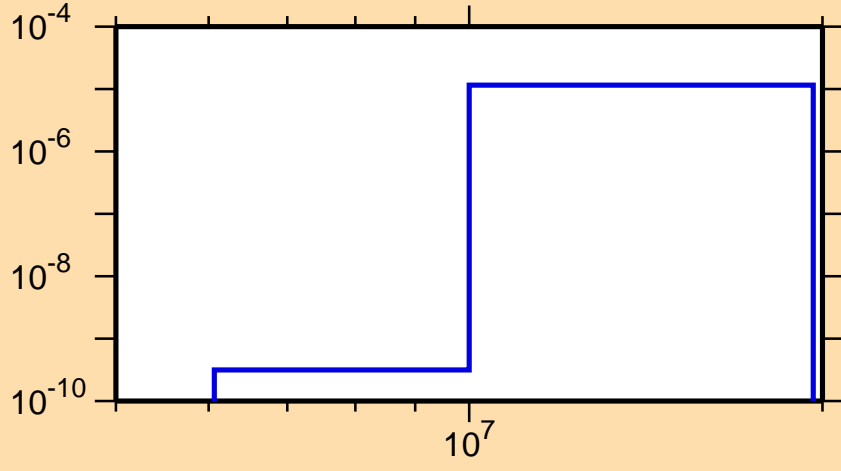
\sigma vs. E for ^{182}\text{Au}(\text{mt } 45)
