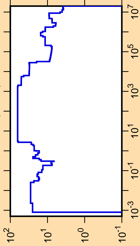
\Delta\sigma/\sigma vs. E for ^{183}\text{Au}(n,\text{tot.})
