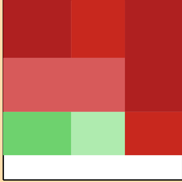
\Delta\sigma/\sigma vs. E for ^{183}\text{Au}(n,\text{el.})
