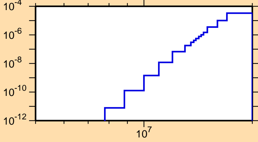
\sigma vs. E for ^{183}\text{Au}(n,\text{He3})
