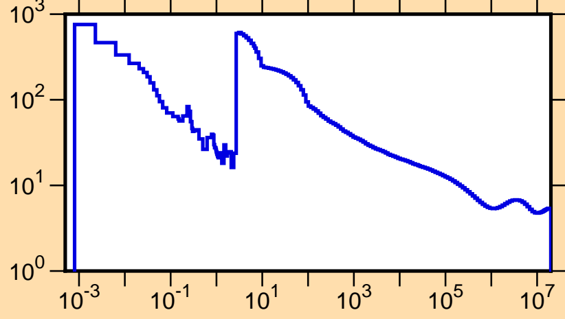
\sigma vs. E for ^{183}\text{Au}(n,\text{tot.})
