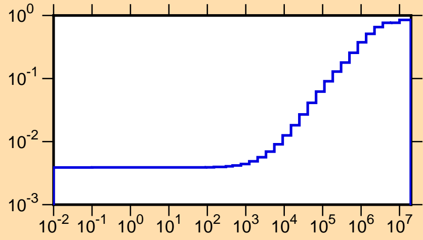
\mu vs. E for ^{183}\text{Au}(\text{mt251})
