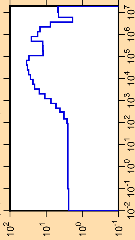
\Delta\mu/\mu vs. E for ^{183}\text{Au}(\text{mt251})
