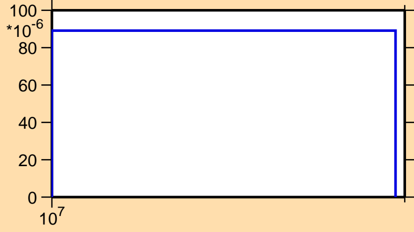
\sigma vs. E for ^{183}\text{Au}(n,2np)
