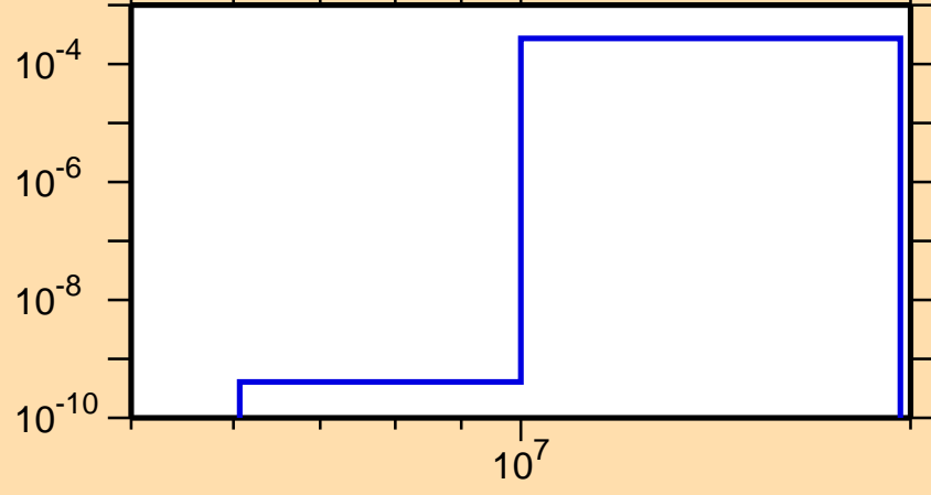
\sigma vs. E for ^{183}\text{Au}(n,t)
