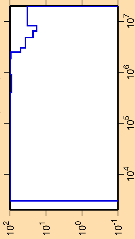
\Delta\sigma/\sigma vs. E for ^{183}\text{Au}(n,\text{inel.})
