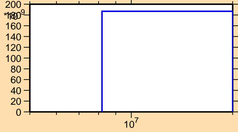
\sigma vs. E for ^{183}\text{Au}(n,\text{nd})
