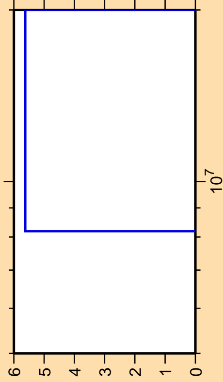
\Delta\sigma/\sigma vs. E for ^{183}\text{Au}(\text{mt } 34)
