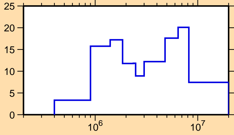
\Delta\sigma/\sigma vs. E for ^{183}\text{Au}(n,el.)
