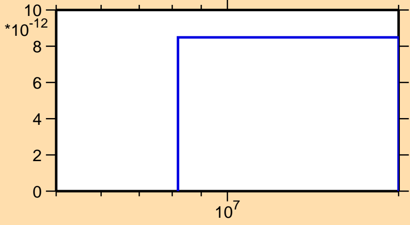
\sigma vs. E for ^{183}\text{Au}(n,\text{pt})
