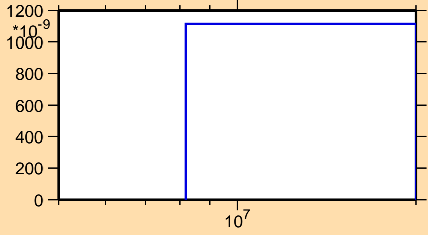
\sigma vs. E for ^{183}\text{Au}(n,2n\alpha)
