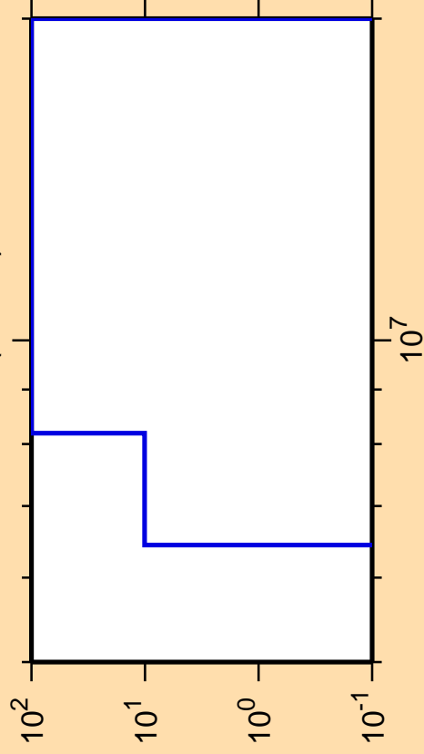
\Delta\sigma/\sigma vs. E for ^{183}\text{Au}(\text{mt } 45)
