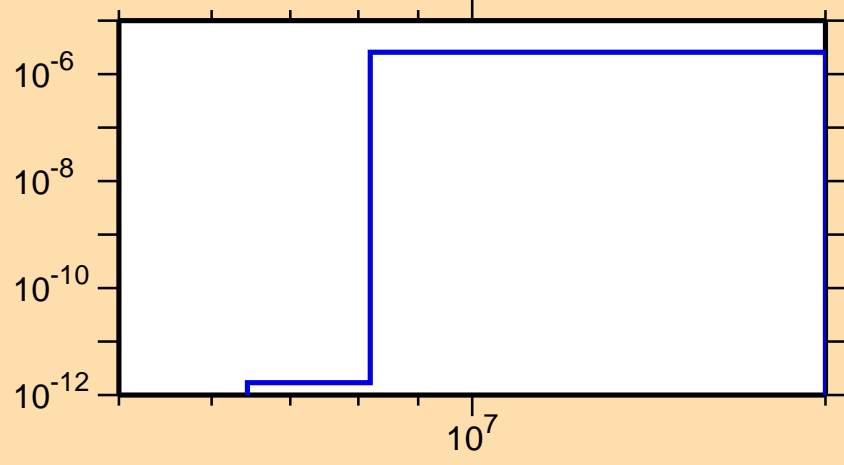
\sigma vs. E for ^{183}\text{Au}(\text{mt } 45)
