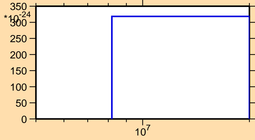
\sigma vs. E for ^{183}\text{Au}(\text{mt } 42)
