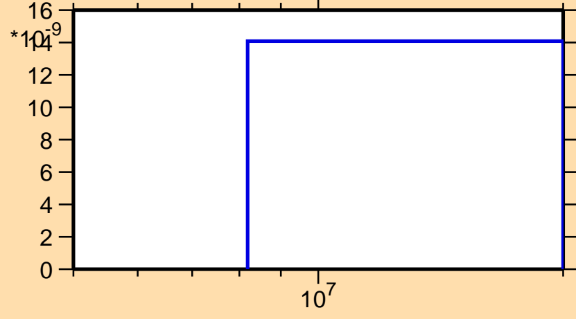
\sigma vs. E for ^{183}\text{Au}(n,\text{pd})
