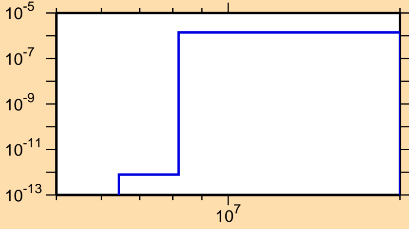
\sigma vs. E for ^{183}\text{Au}(n,\text{He3})
