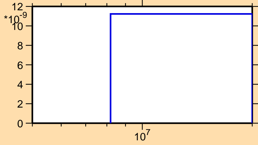
\sigma vs. E for ^{183}\text{Au}(\text{mt117})
