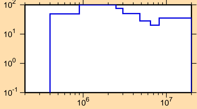
\Delta\sigma/\sigma vs. E for ^{183}\text{Au}(n,ncont.)
