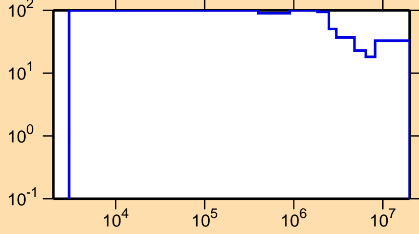
\Delta\sigma/\sigma vs. E for ^{183}\text{Au}(n,\text{inel.})
