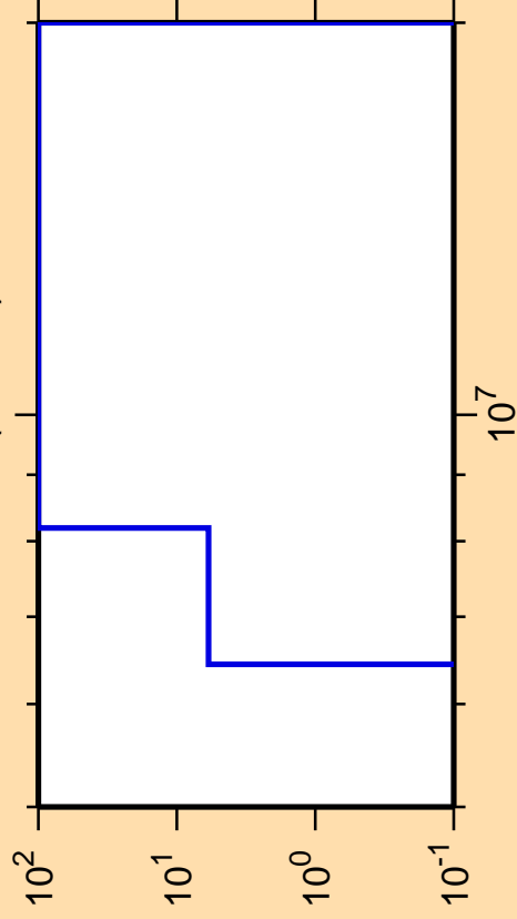
\Delta\sigma/\sigma vs. E for ^{183}\text{Au}(n,\text{He3})
